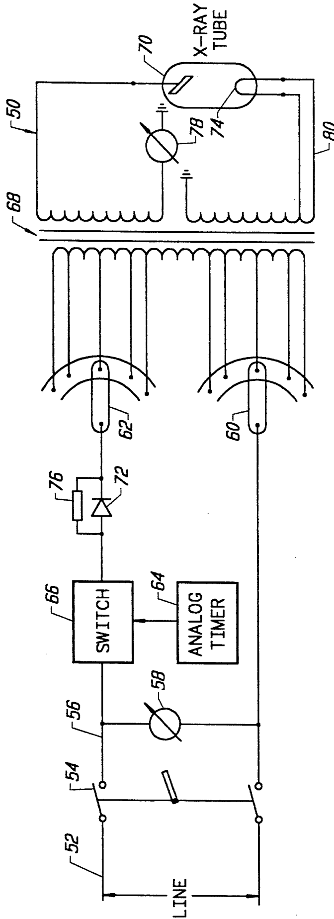
FIG. 2 (PRIOR ART)
