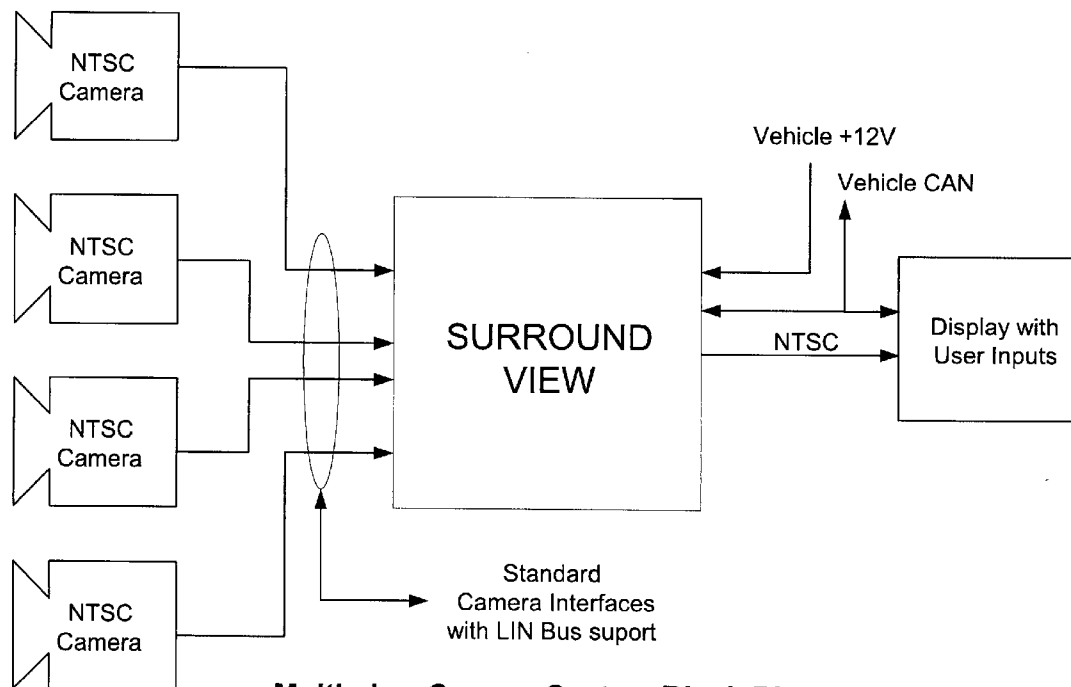
Multi-view Camera System Block Diagram
