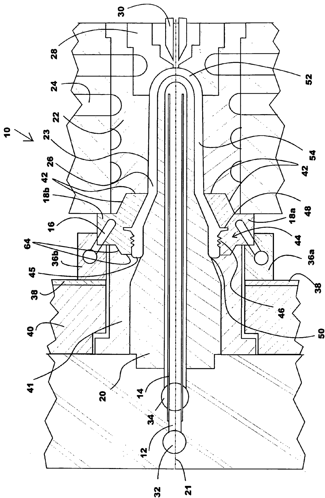
Figure 1. (Prior Art)
