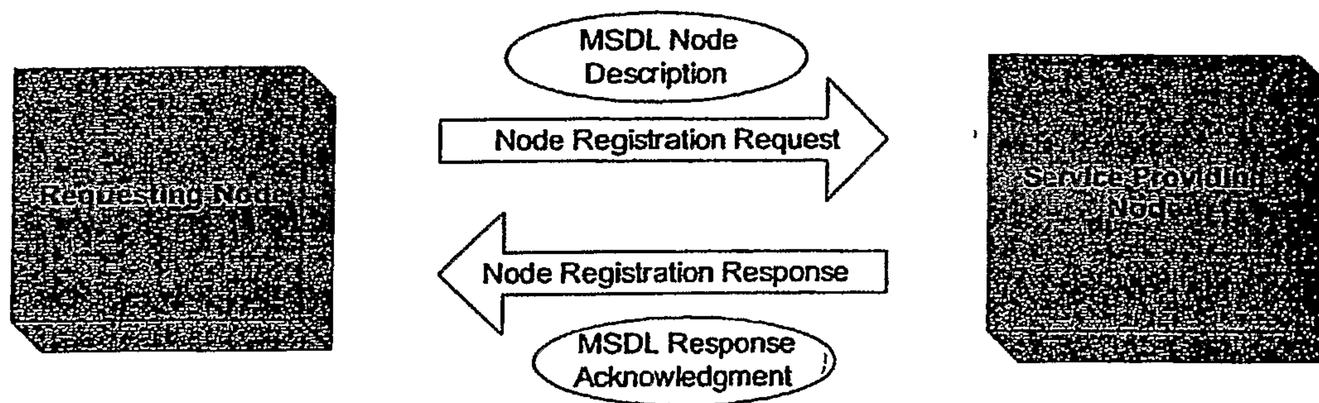
Service Discovery – Node Registration
