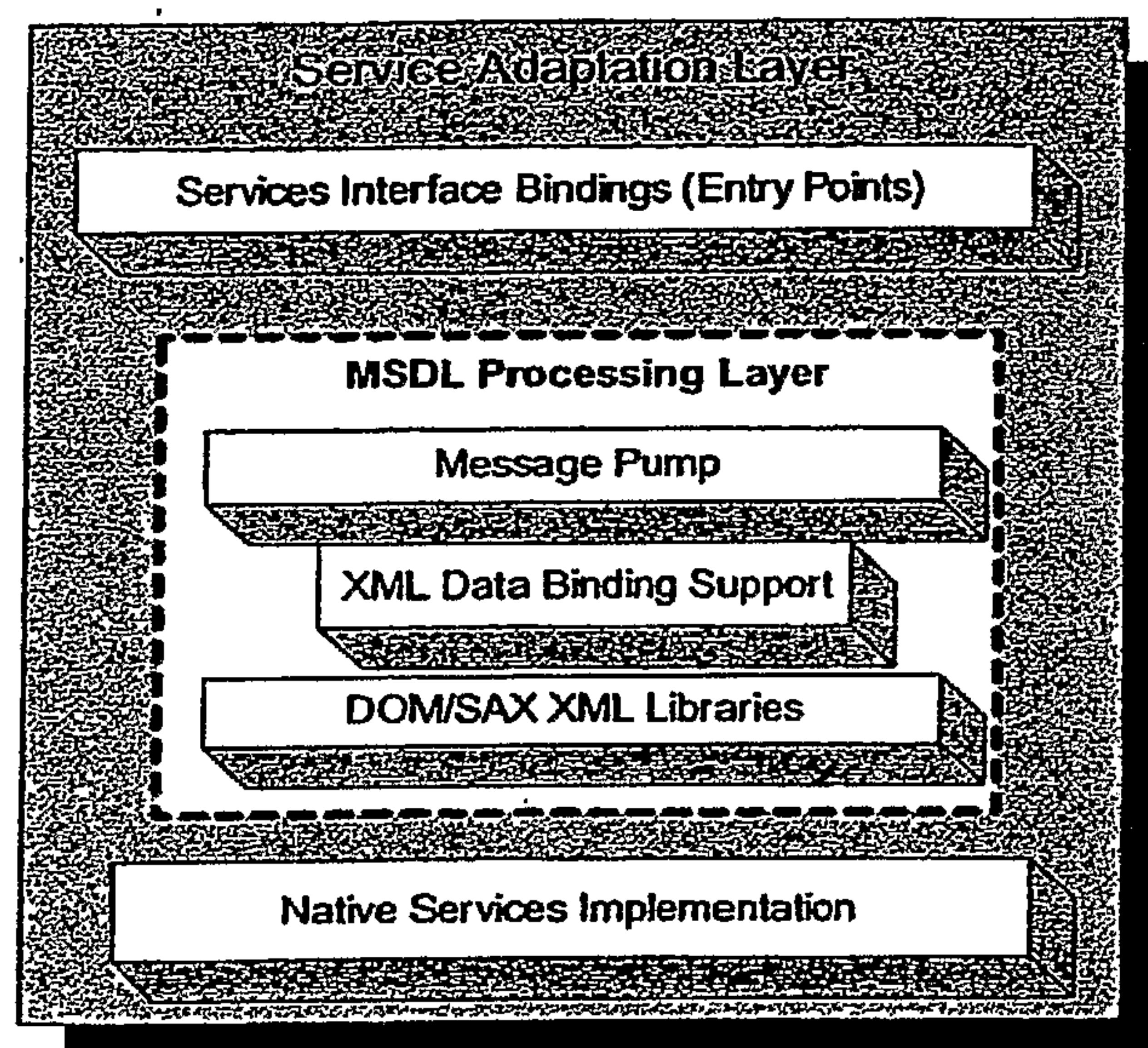
Service Adaptation Layer
