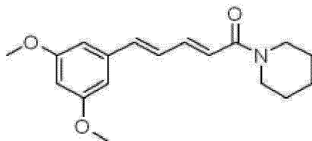
Chemical Formula 10
