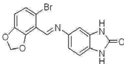
Chemical Formula 14
