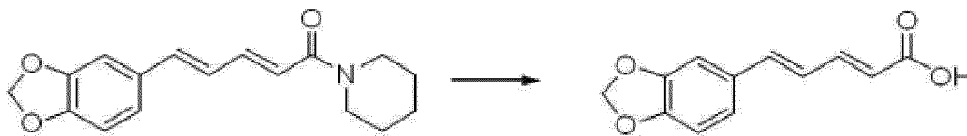
Piperine
