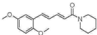
Chemical Formula 8
