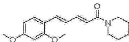
Chemical Formula 8
