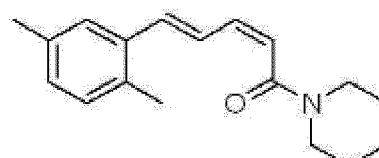
Chemical Formula 12
