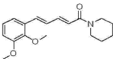
Chemical Formula 7
