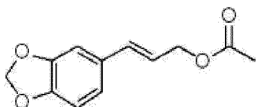
Chemical Formula 5
