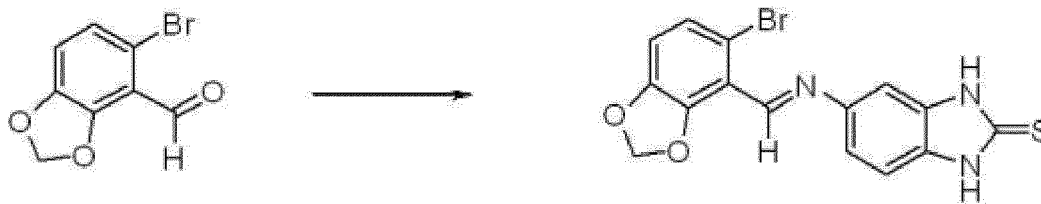
(E)-5-((5-bromobenzo[d][1,3]dioxol-4-yl)methyleneamino)-1H-benzo[d]imidazole-2(3H)-thione (SKKU-S-02)
