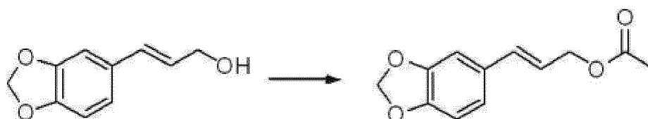
(E)-3-benz[d][1,3]dioxol-5-ylallyl acetate (LJ-2196)
