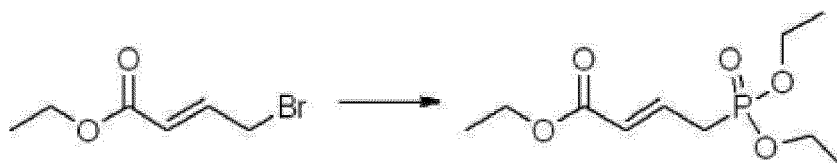
(E)-ethyl 4-(diethoxyphosphoryl)but-2-enoate
