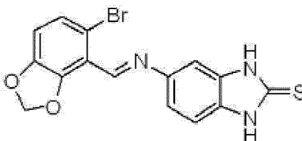
Chemical Formula 15
