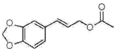
Chemical Formula 6
