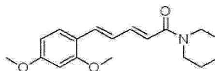
Chemical Formula 10
