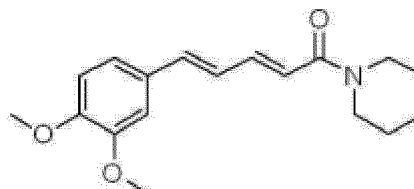
Chemical Formula 9
