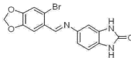
Chemical Formula 15
