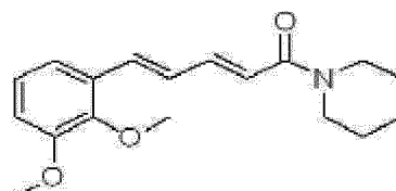
Chemical Formula 9
