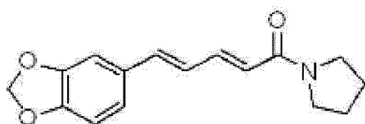
Chemical Formula 7
