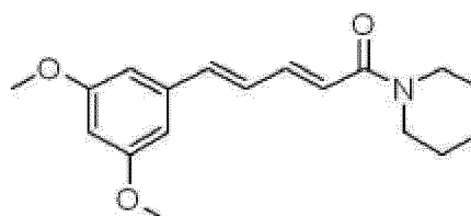
Chemical Formula 10
