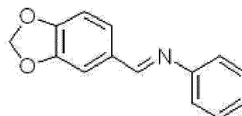
Chemical Formula 6
