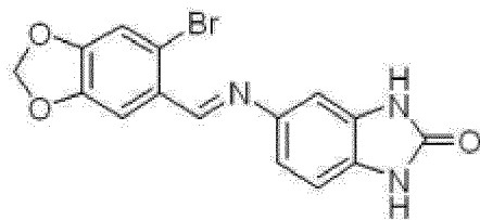
Chemical Formula 15
