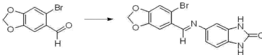
(E)-5-((6-bromobenzo[d][1,3]dioxol-5-yl)methyleneamino)-1H-benzo[d]imidazole-2(3H)-one (LJ-2527)
