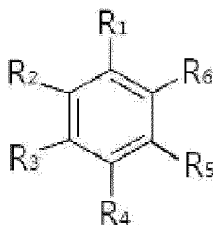
Chemical Formula 1
