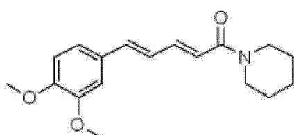
Chemical Formula 11
