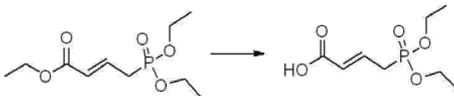
(E)-4-(diethoxyphosphoryl)but-2-enoate
