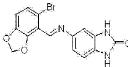
Chemical Formula 14
