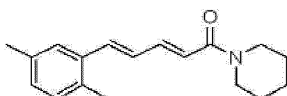
Chemical Formula 11
