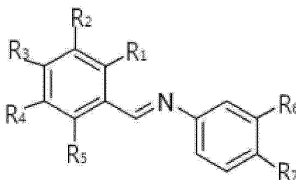
Chemical Formula 2
