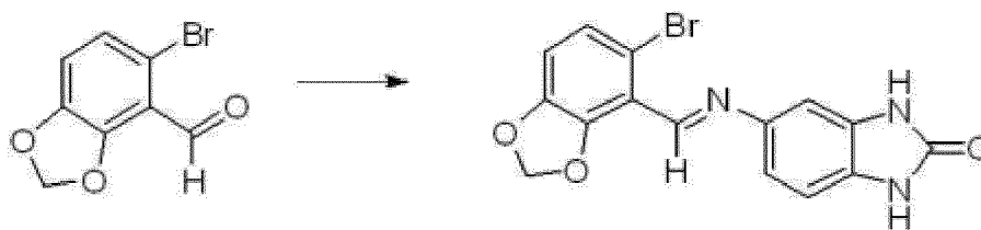
(E)-5-((5-bromobenzo[d][1,3]dioxol-4-yl)methyleneamino)-1H-benzo[d]imidazole-2(3H)-one (LJ-2529)
