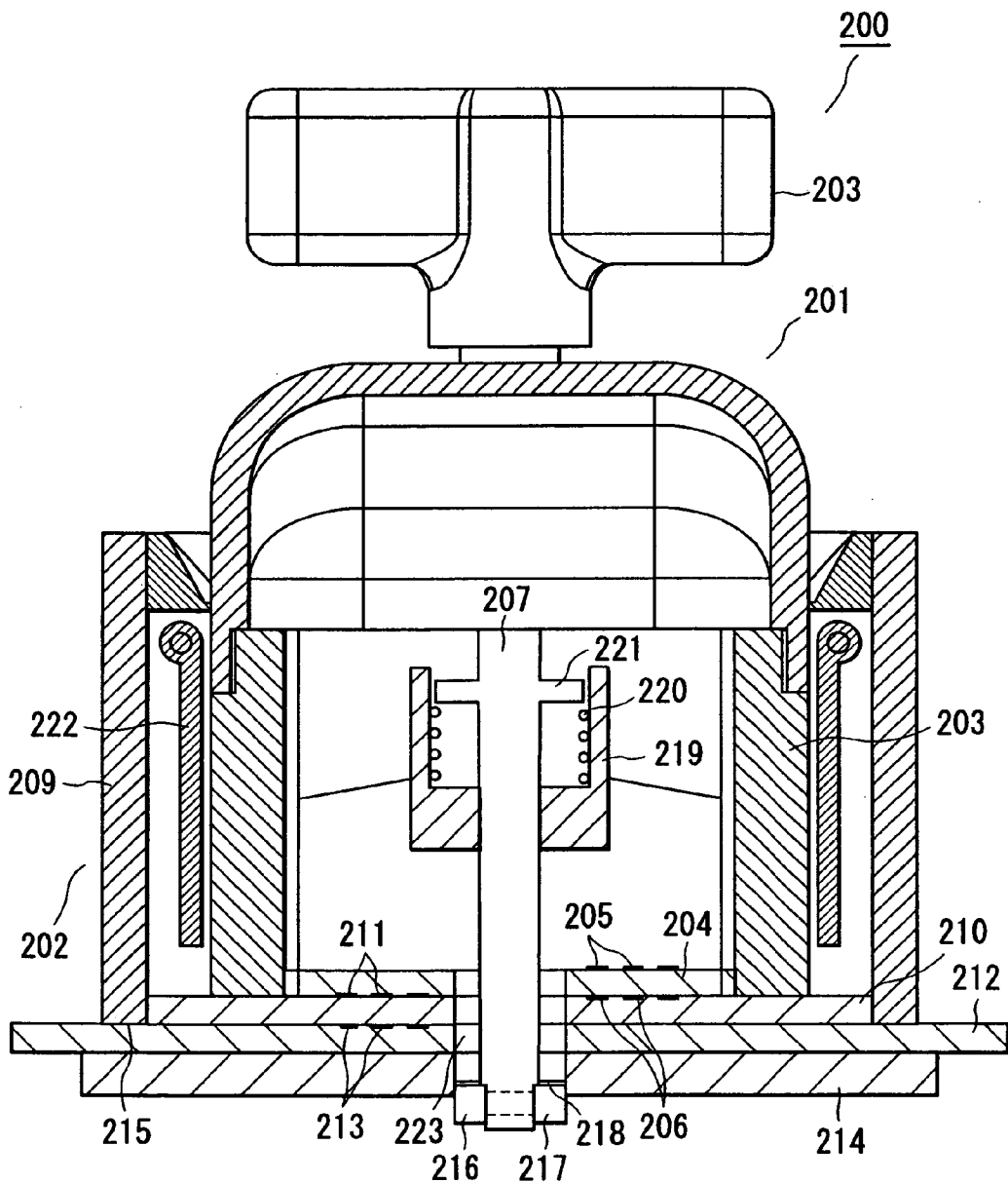
FIG. 12 (PRIOR ART)
