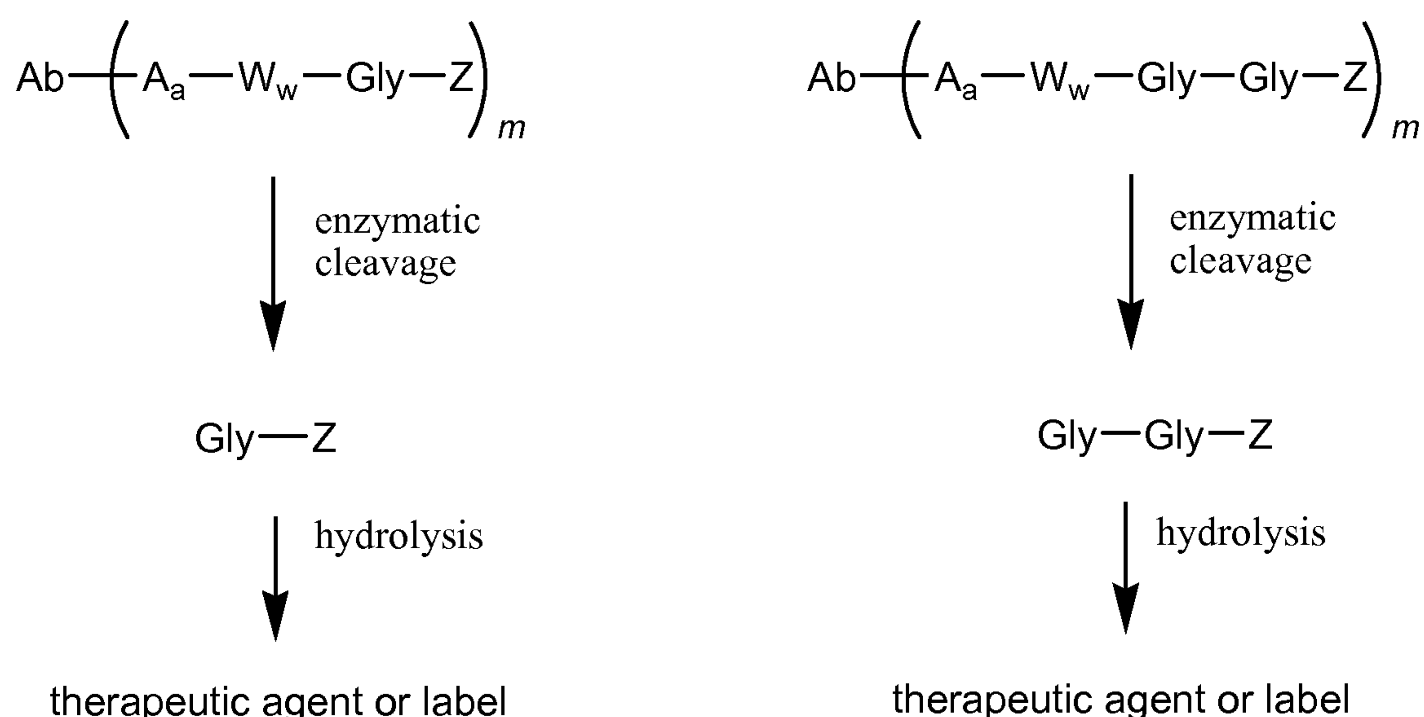
Scheme 1
