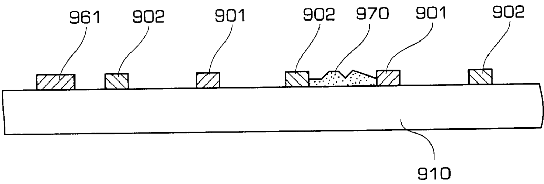
FIG. 6 PRIOR ART
