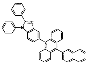
Compound B
