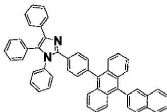
Compound (2)
