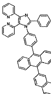
Compound (3)
