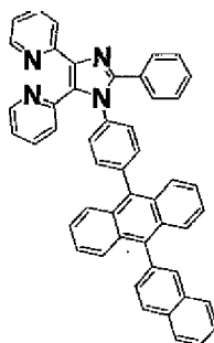
Compound (3)
