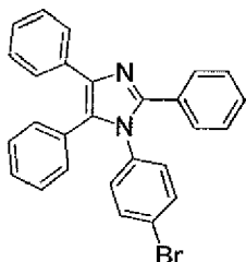
Intermediate 1
