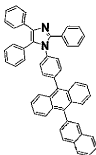
Compound (1)
