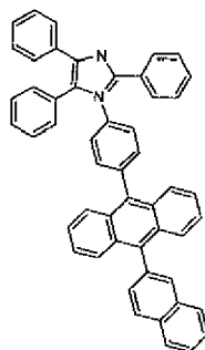
Compound (1)
