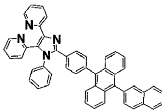
Compound (4)
