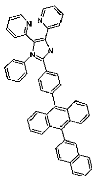
Compound (4)
