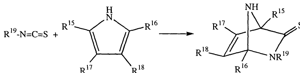
Scheme 2
