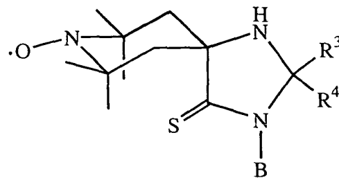
(VIb)
