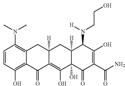
Compound 12— R_4=NH-CH_2CH_2CH_2-OH , up bond at minocycline position
