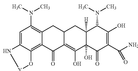
Compound 3
