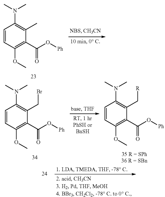
Scheme 10.
