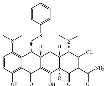
Compound 14— R_6=CH_2-S-aryl (phenyl), down bond at position 4.
