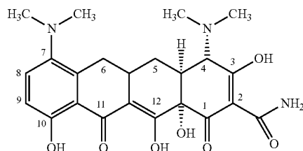
Minocycline
