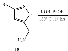
Scheme 8.
