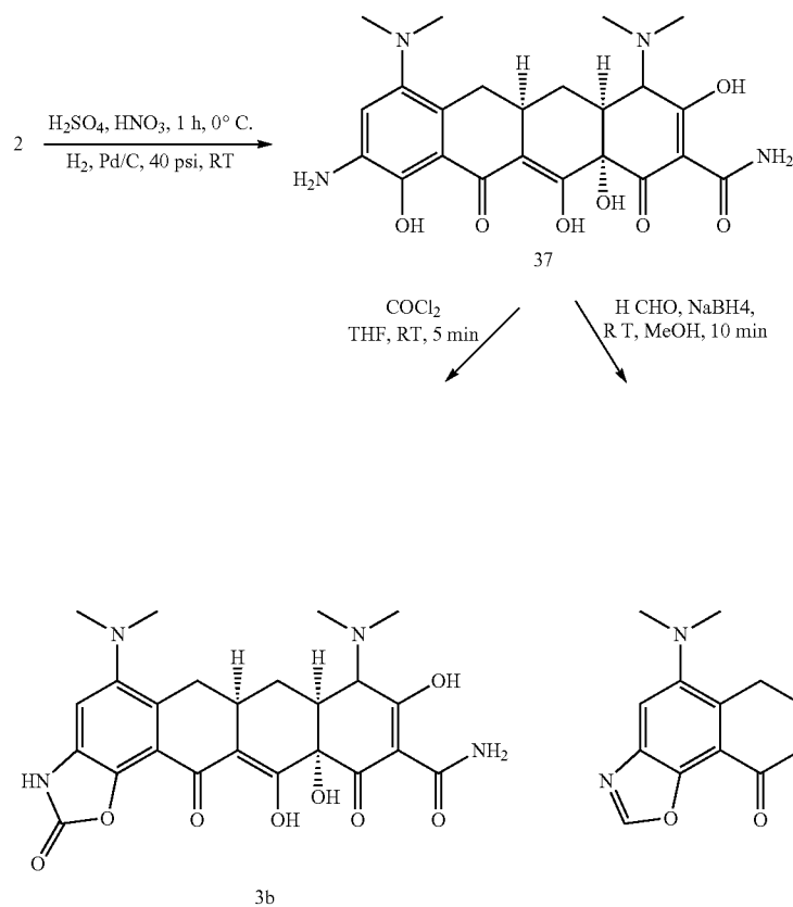
Scheme 11.
