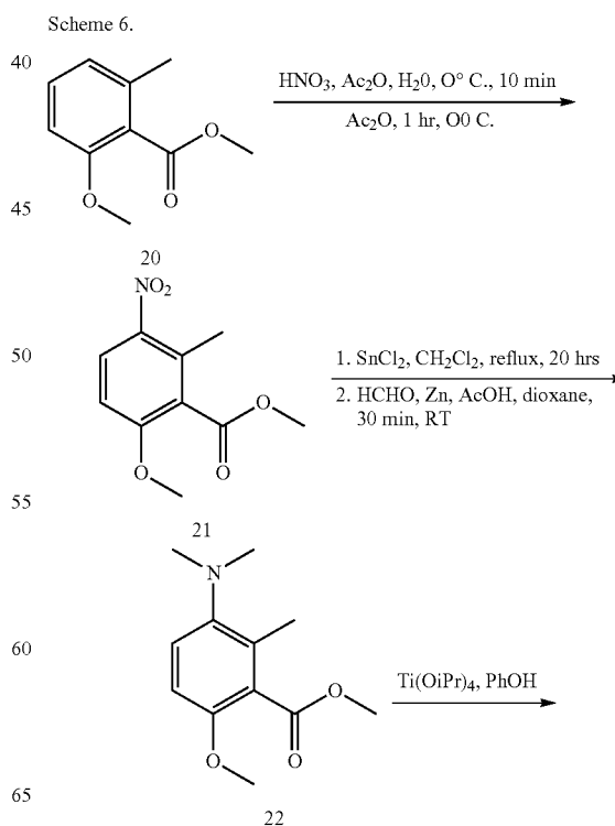
Scheme 6.
