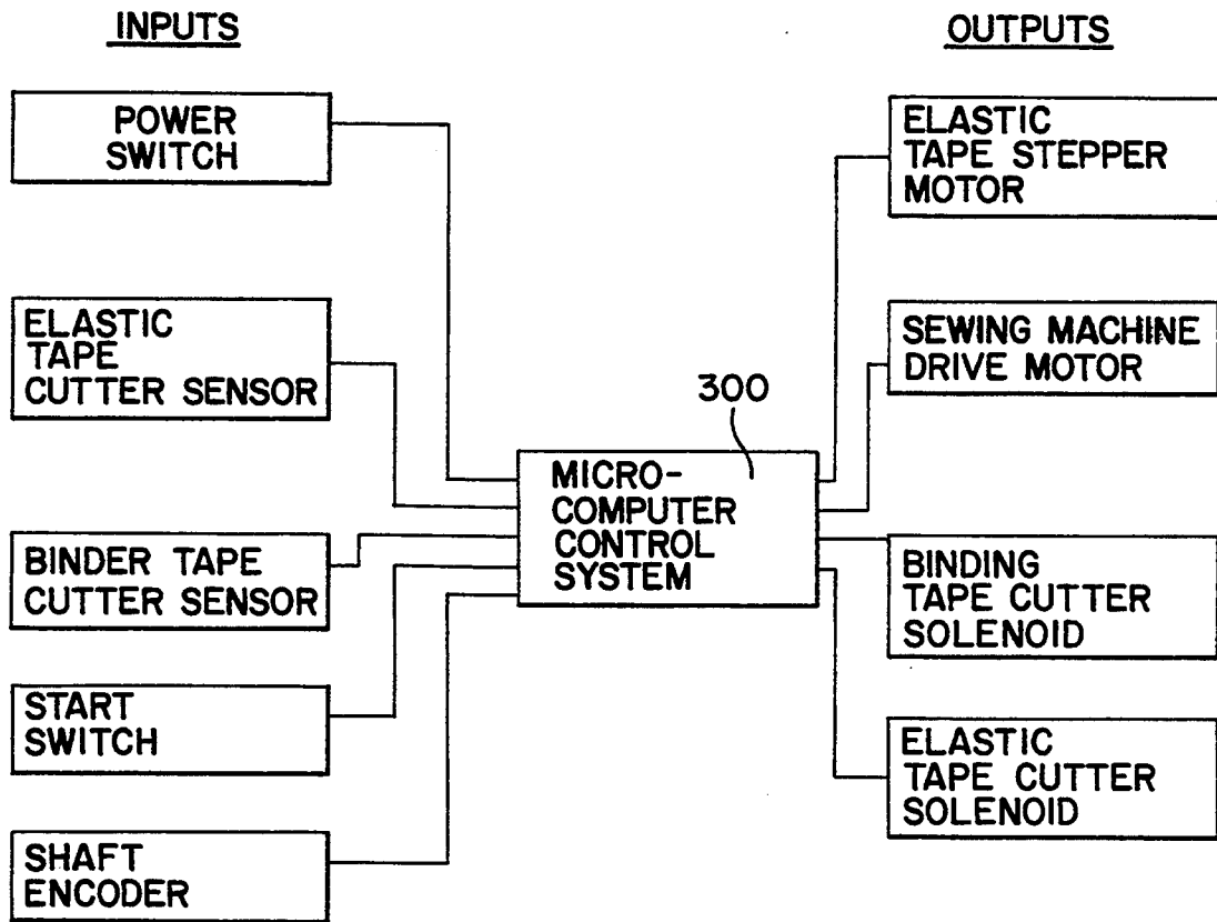
BLOCK DIAGRAM OF CONTROL SYSTEM
