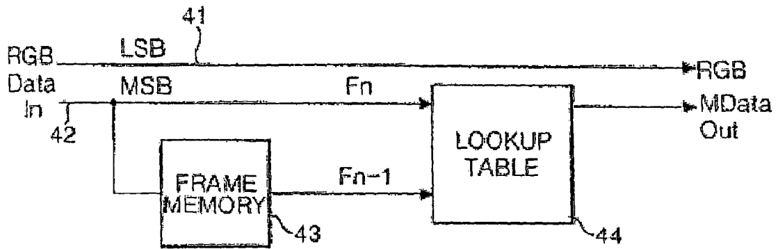
FIG. 4 RELATED ART
