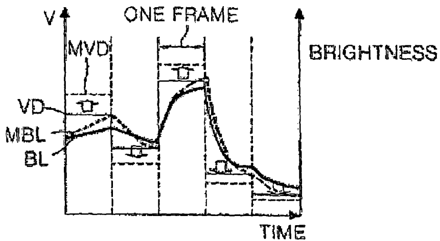
FIG. 2 RELATED ART
