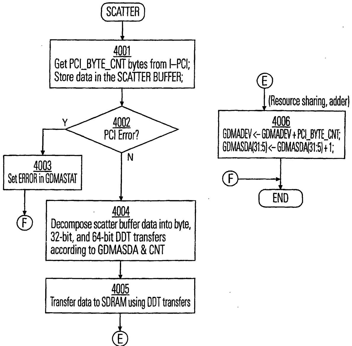
FIGURE 1-19 SCATTER OPERATION
