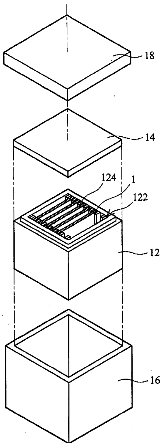
FIG. 1 ( RELATED ART )
