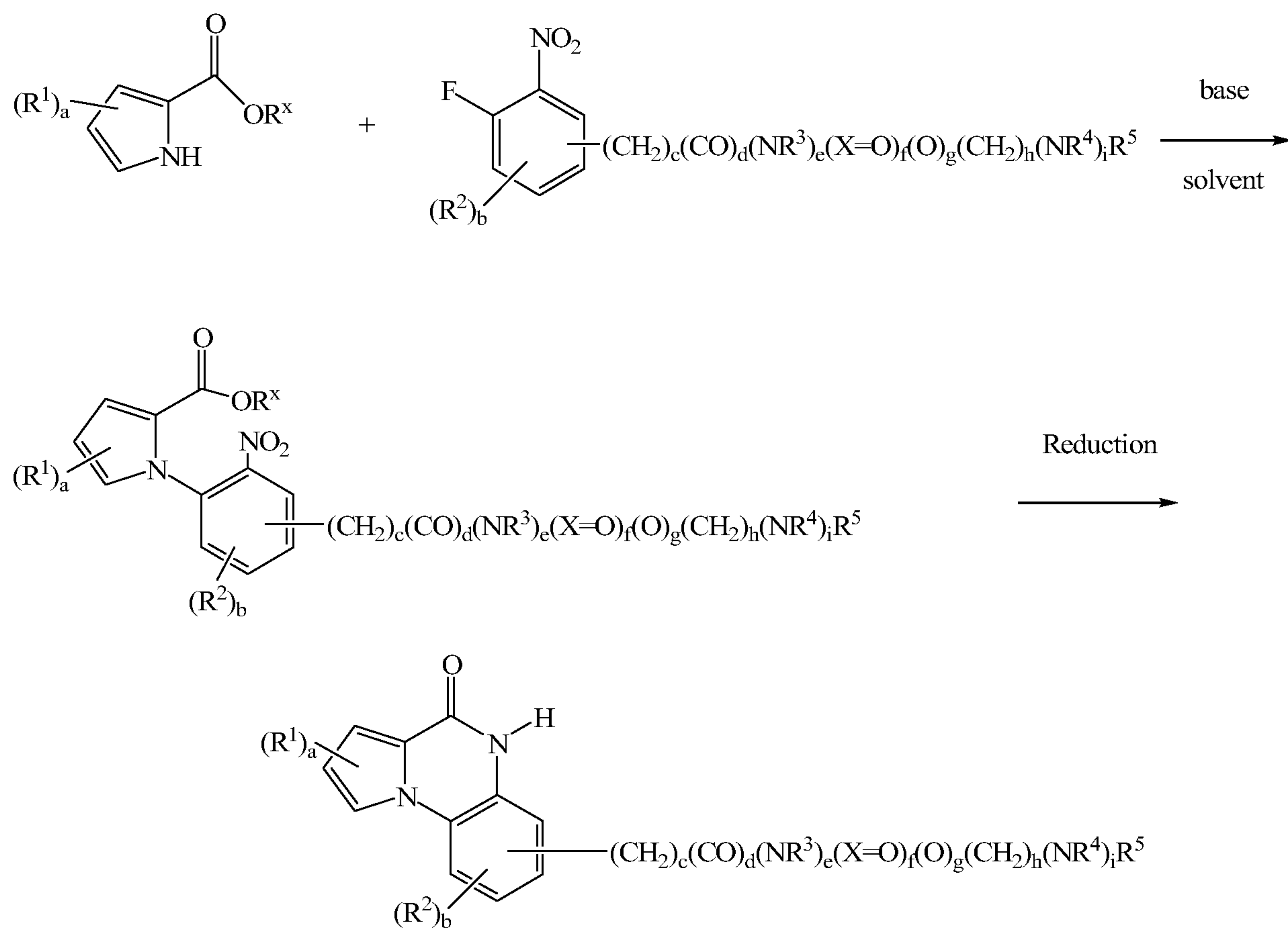
Scheme 1
