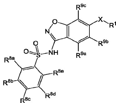
Formula (II);
