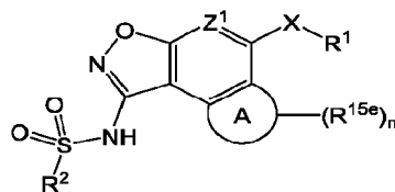
Formula (V),
