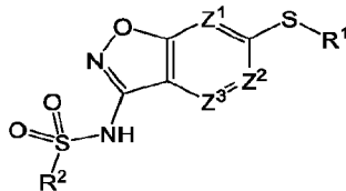
Formula (IV),
