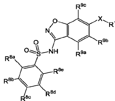
Formula (III);
