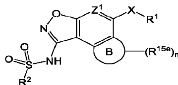
Formula (VI),
