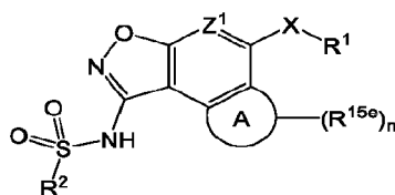
Formula (V),
