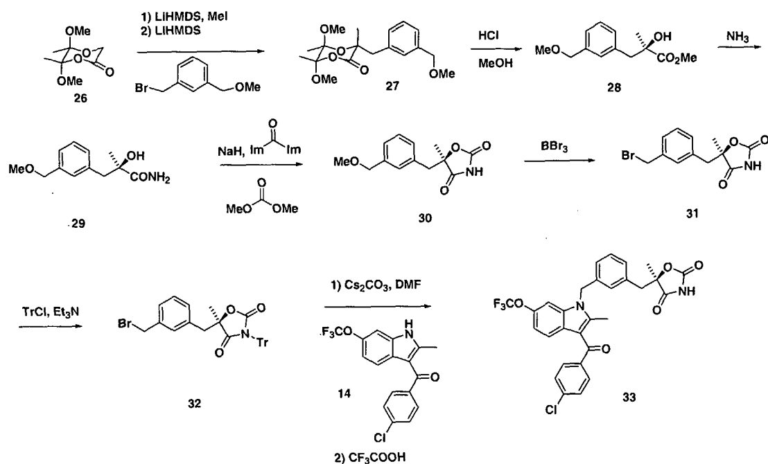
Scheme 8.
