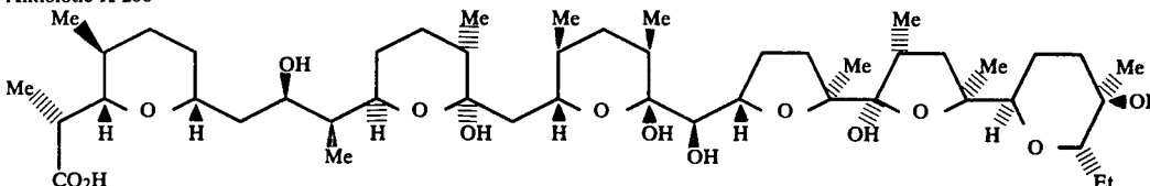
Antibiotic X-206
