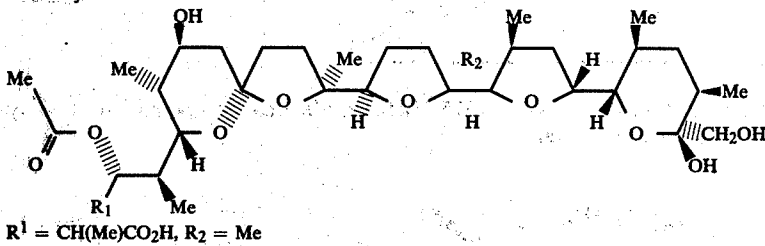
Laidlomycin
