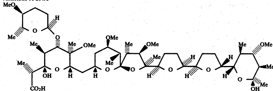
Antibiotic A-204A
