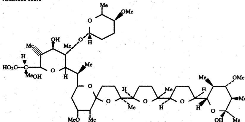
Antibiotic 38295
