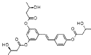
Compound 7: [4-[(E)-2-[3,5-bis[(3R)-3-hydroxybutanoyloxy]phenyl]vinyl]phenyl] (3R)-3-hydroxybutanoate
