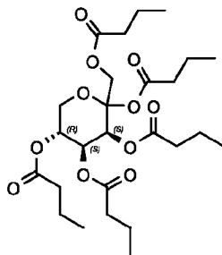
Compound 163: [(3S,4S,5R)-2,3,4,5-tetrakis(butanoyloxy)oxan-2-yl]methyl butanoate
