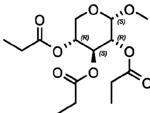
Compound 105: (2S,3R,4S,5R)-2-methoxy-4,5-bis(propionyloxy)oxan-3-yl propanoate
