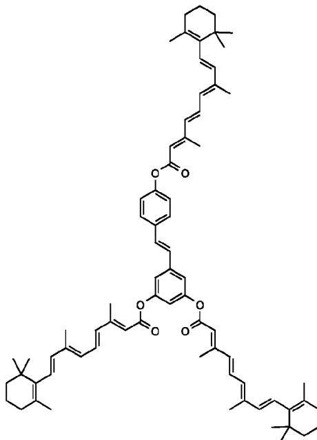
Compound 261: 3-[(2E,4E,6E,8E)-3,7-dimethyl-9-(2,6,6-trimethylcyclohex-1-en-1-yl)nona-2,4,6,8-tetraenoyl]oxy-5-[(1E)-2-(4-[(2E,4E,6E,8E)-3,7-dimethyl-9-(2,6,6-trimethylcyclohex-1-en-1-yl)nona-2,4,6,8-tetraenoyl]oxy}phenyl)ethenyl]phenyl (2E,4E,6E,8E)-3,7-dimethyl-9-(2,6,6-trimethylcyclohex-1-en-1-yl)nona-2,4,6,8-tetraenoate
