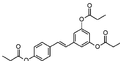
Compound 9: [4-[(E)-2-[3,5-di(propanoyloxy)phenyl]vinyl]phenyl] propanoate
