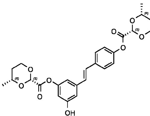
Compound 256: 4-[(1E)-2-{3-hydroxy-5-[(2S,4R)-4-methyl-1,3-dioxane-2-carboxyloxy]phenyl}ethenyl]phenyl (2S,4R)-4-methyl-1,3-dioxane-2-carboxylate
