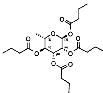
Compound 152: (2S,3R,4R,5S,6S)-3,4,5-tris(butanoyloxy)-6-methyloxan-2-yl butanoate
