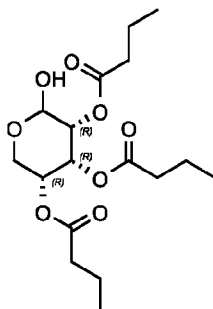
Compound 185: (3R,4R,5R)-4,5-bis(butanoyloxy)-2-hydroxyoxan-3-yl butanoate
