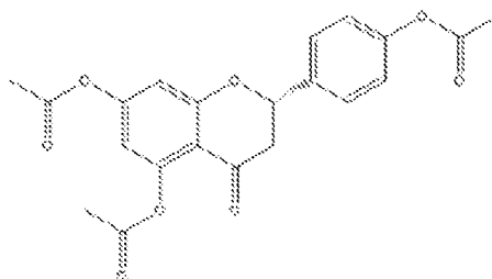
Compound 21: (S)-2-(4-acetoxypheyl)-4-oxochroman-5,7-diyl diacetate
