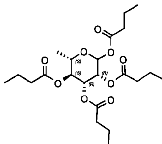
Compound 174: (3R,4R,5S,6S)-3,4,5-tris(butanoyloxy)-6-methyloxan-2-yl butanoate
