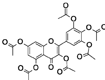
Compound 23: [3,5-diacetoxy-4-oxo-2-(3,4,5-triacetoxyphenyl)chromen-7-yl] acetate
