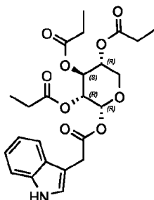
Compound 149: (2R,3R,4S,5R)-2-[[2-(1H-indol-3-yl)acetyl]oxy]-4,5-bis(propanoyloxy)oxan-3-yl propanoate
