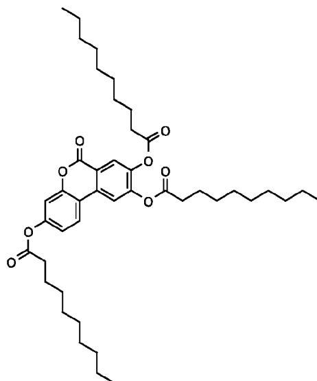
Compound 245: 8,9-bis(decanyloxy)-6-oxo-6H-benzo[c]chromen-3-yl decanoate
