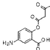
Compound 36: 5-amino-2-(3-oxobutanoyloxy)benzoic acid
