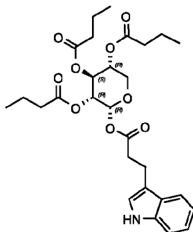
15 Compound 128: (2R,3R,4S,5R)-4,5-bis(butanoyloxy)-2-[[3-(1H-indol-3-yl)propanoyl]oxy]oxan-3-yl butanoate
