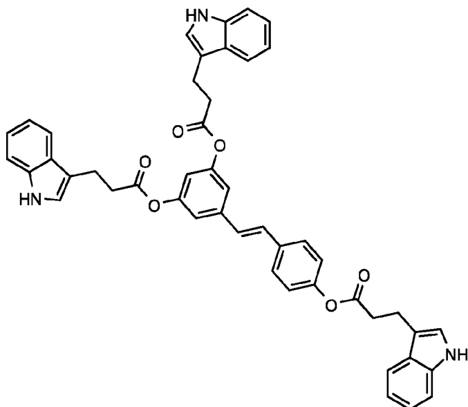
Compound 259: 4-[(1E)-2-[3,5-bis({[3-(1H-indol-3-yl)propanoyl]oxy})phenyl]ethenyl]phenyl 3-(1H-indol-3-yl)propanoate
