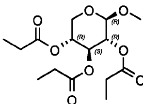
Compound 106: (2R,3R,4S,5R)-2-methoxy-4,5-bis(propionyloxy)oxan-3-yl propanoate
