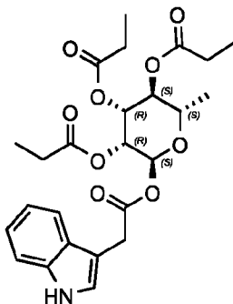
Compound 147: (2S,3R,4R,5S,6S)-2-[[2-(1H-indol-3-yl)acetyl]oxy]-6-methyl-4,5-bis(propanoyloxy)oxan-3-yl propanoate
