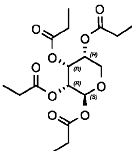
Compound 136: (2S,3R,4R,5R)-3,4,5-tris(propanoyloxy)oxan-2-yl propanoate
