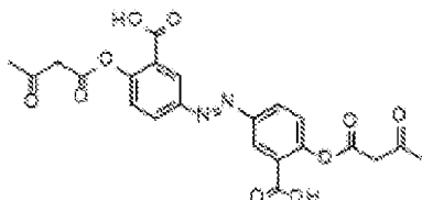
25 Compound 35: 5-[(E)-[3-carboxy-4-(3-oxobutanoyloxy)phenyl]azo]-2-(3-oxobutanoyloxy)benzoic acid
