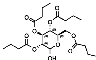
Compound 165: [(2R,3R,4S,5R)-3,4,5-tris(butanoyloxy)-6-hydroxyoxan-2-yl]methyl butanoate
