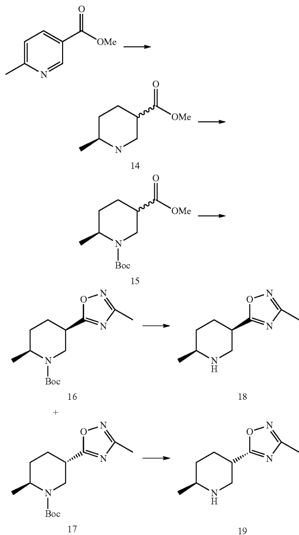
Scheme 4
