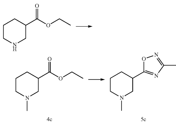
N-Methyl-ethyl nipecotate (4c)
