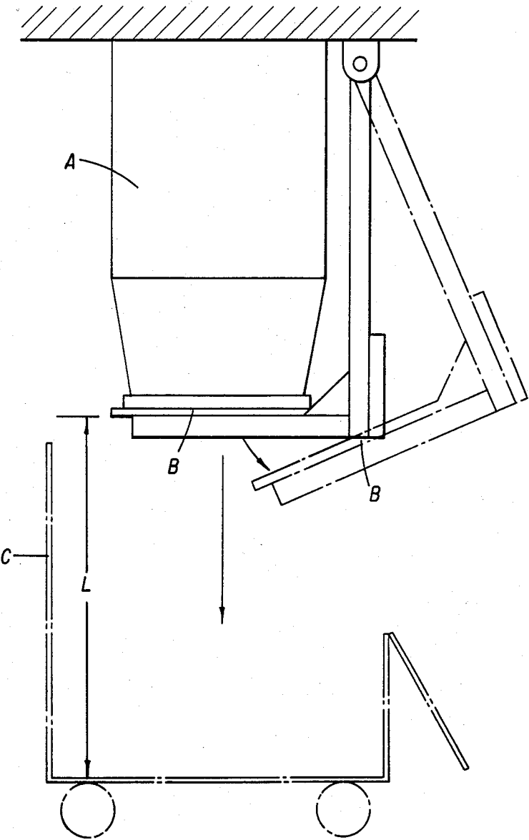
FIG. 2 PRIOR ART
