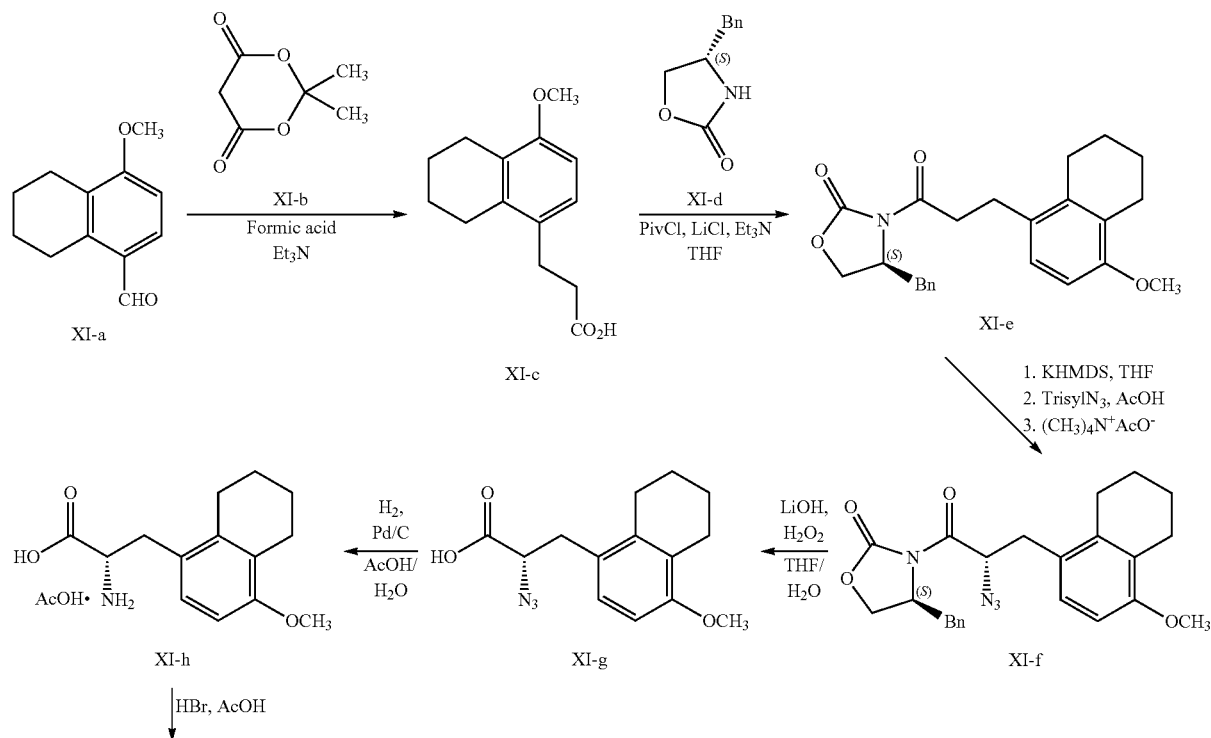
Scheme XI 3,5-diamino-N—(N-(4-(6-((S)-3-amino-2-(3-(bis((2S,3R,4R,5R)-2,3,4,5,6-pentahydroxyhexyl)amino)propylamino)-3-oxopropyl)-5,6,7,8-tetrahydronaphthalen-1-yl)butyl)carbamimidoyl)-6-chloropyrazine-2-carboxamide
