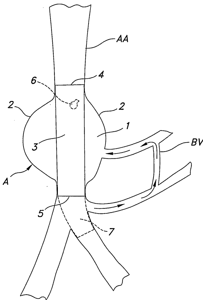
FIG. 1 (PRIOR ART)
