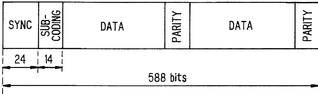
FRAME STRUCTURE
