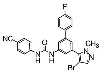
Compound 193
