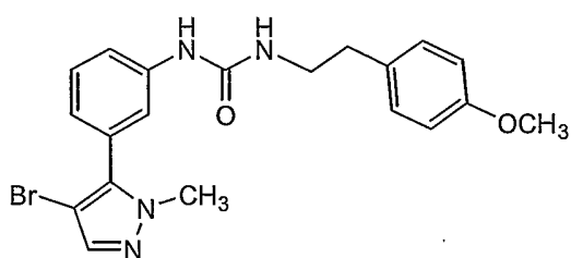
Compound 38
