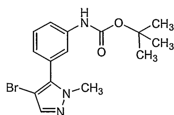
Compound 39
