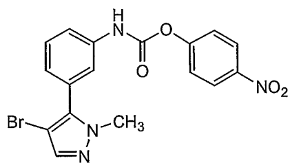
Compound 59
