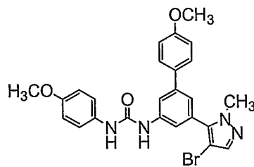
Compound 198
