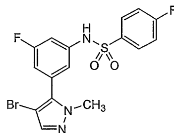
Compound 97
