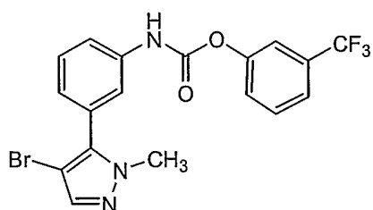
Compound 66
