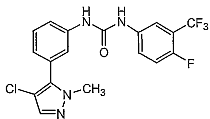
Compound 182
