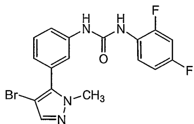
Compound 173
