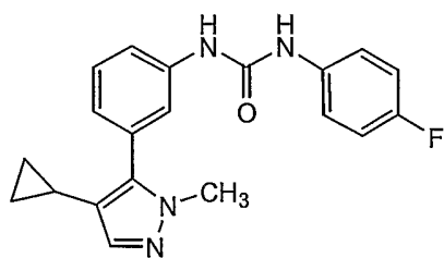
Compound 95
