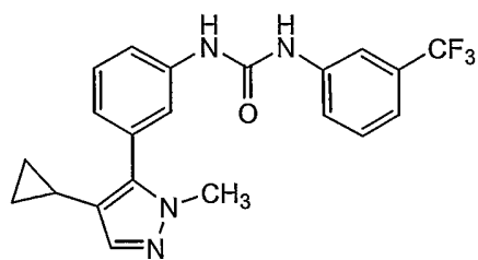
Compound 87
