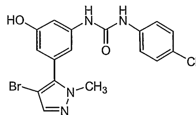
Compound 157
