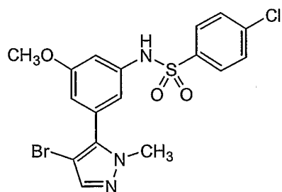
Compound 152
