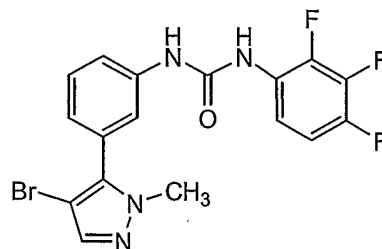
Compound 174
