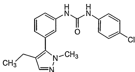
Compound 78
