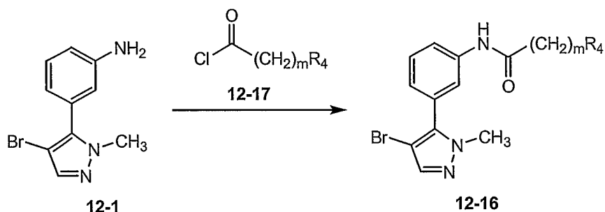
Scheme 12-10
