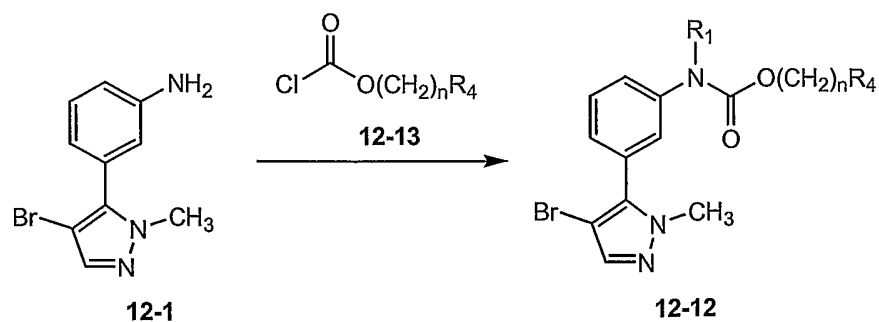
Scheme 12-6
