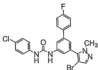
Compound 199
