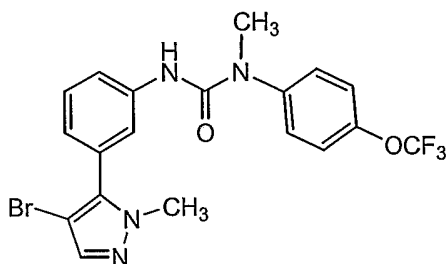
Compound 22
