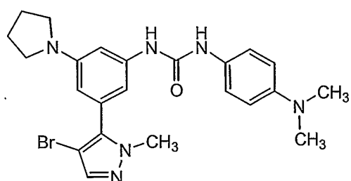
Compound 110
