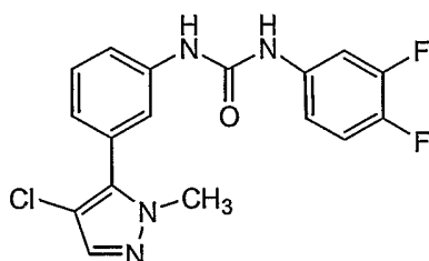
Compound 171
