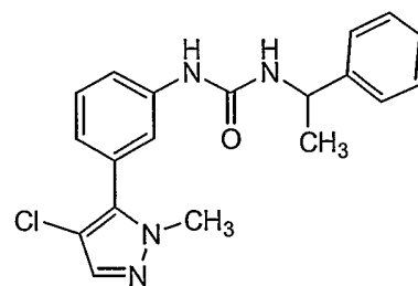
Compound 51
