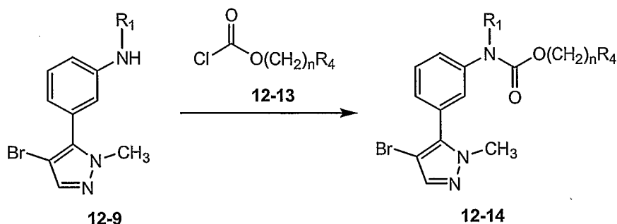
Scheme 12-7
