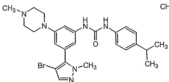
Compound 116
