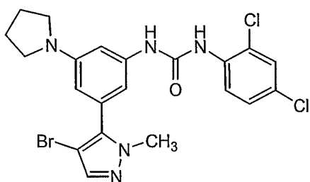
Compound 122
