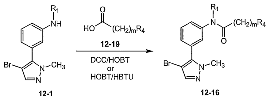
Scheme 12-12
