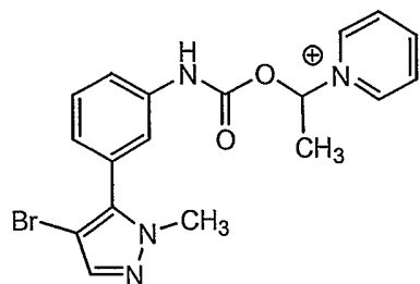
Compound 72
