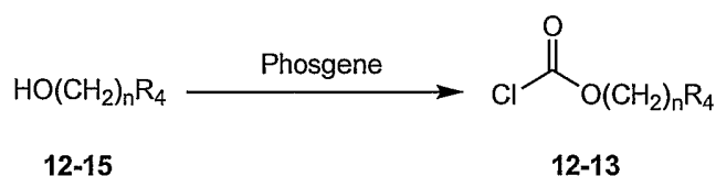
Scheme 12-9
