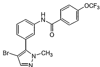
Compound 40
