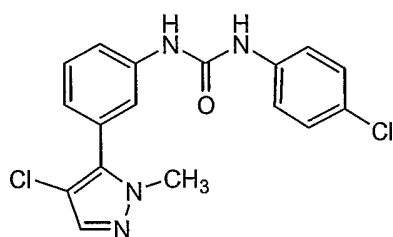
Compound 48
