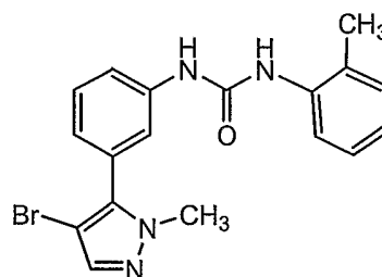
Compound 15
