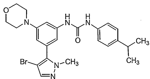
Compound 111
