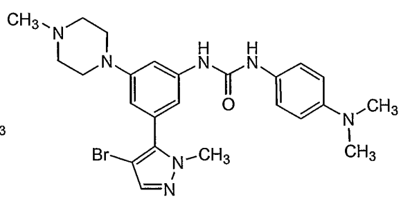
Compound 147
