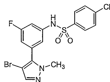
Compound 103
