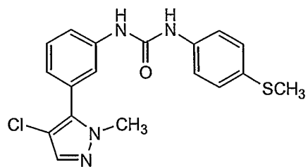
Compound 55
