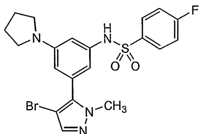
Compound 118
