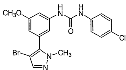
Compound 158
