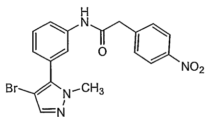
Compound 46
