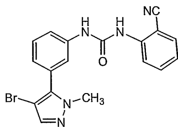
Compound 30
