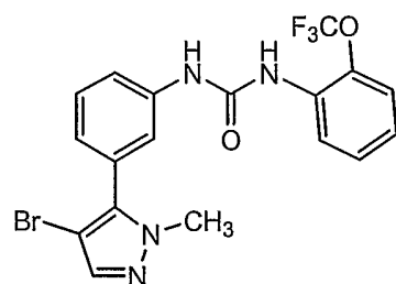
Compound 12
