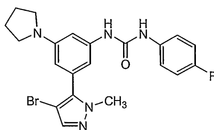
Compound 131
