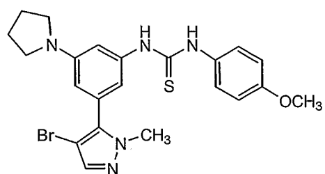
Compound 115
