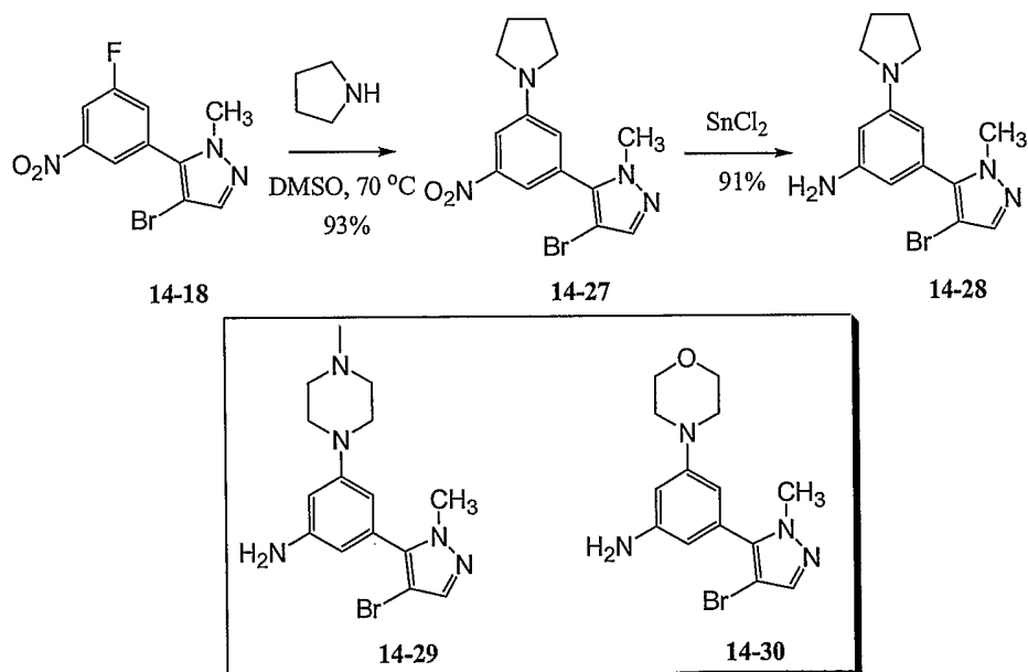
Scheme 14-7
