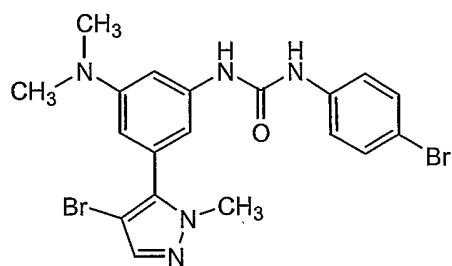
Compound 105
