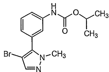
Compound 73
