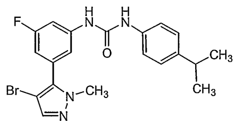
Compound 99
