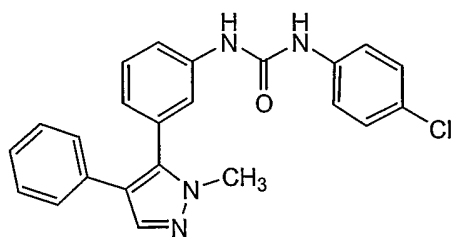
Compound 80
