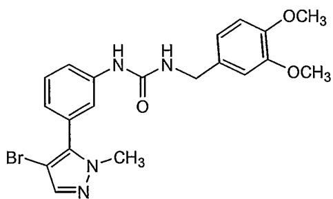
Compound 34
