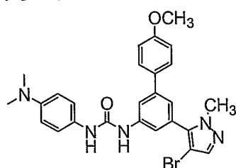
Compound 185
