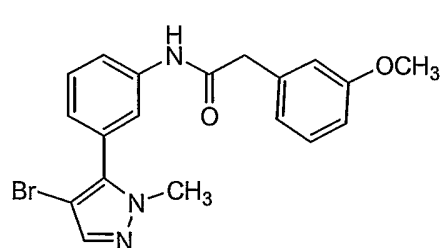
Compound 44
