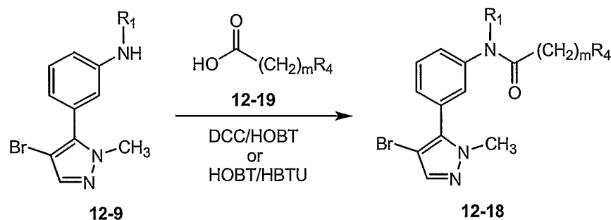
Scheme 12-13
