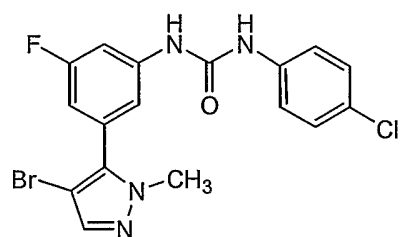
Compound 96
