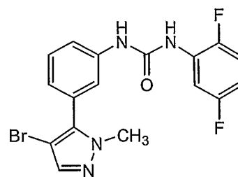
Compound 166
