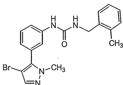
Compound 36
