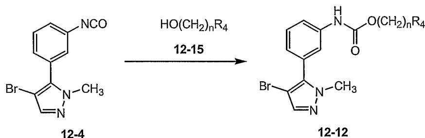
Scheme 12-8
