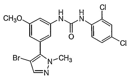
Compound 159
