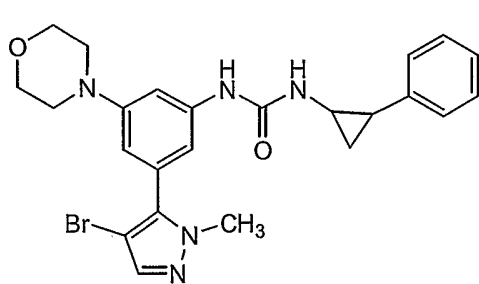
Compound 126
