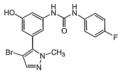
Compound 151
