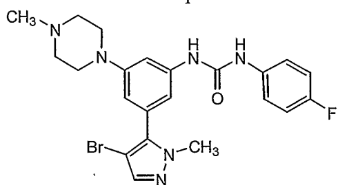
Compound 124
