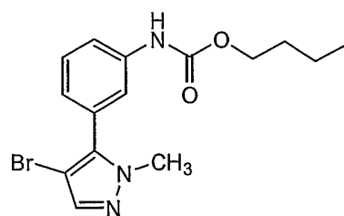
Compound 63
