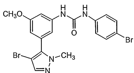
Compound 154
