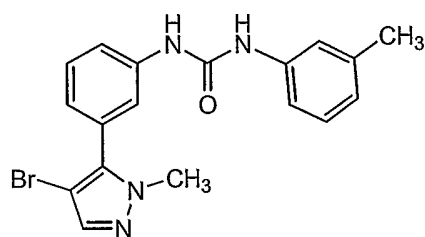
Compound 21
