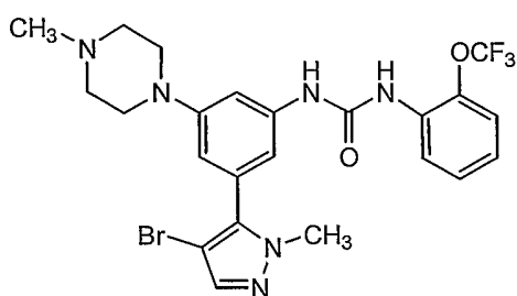
Compound 114
