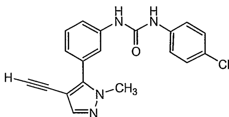
Compound 90
