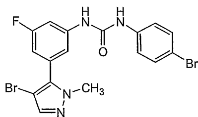
Compound 98
