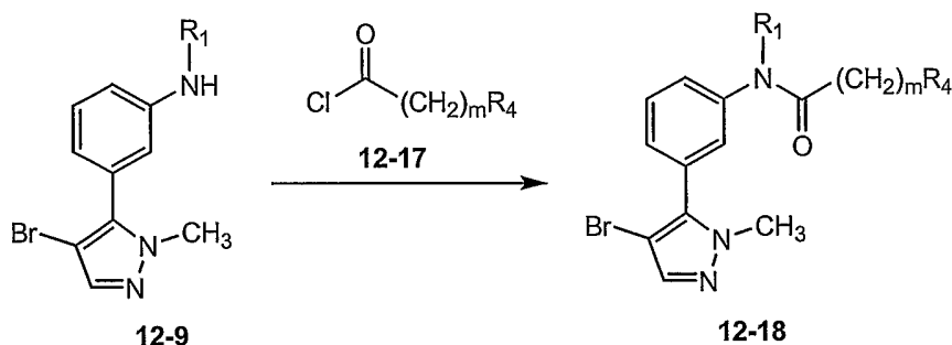
Scheme 12-11
