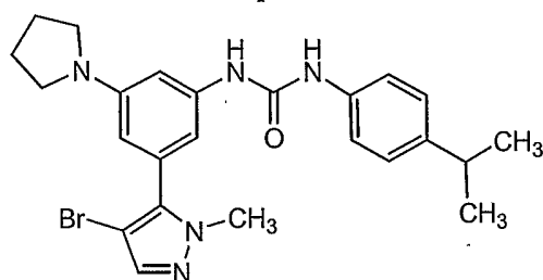
Compound 148
