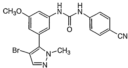
Compound 163
