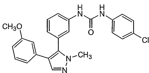
Compound 82
