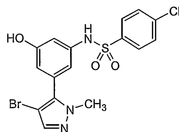
Compound 155
