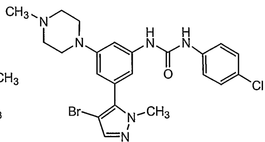
Compound 117
