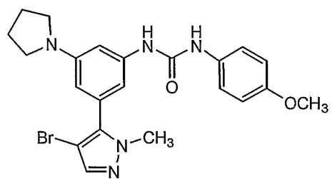
Compound 125
