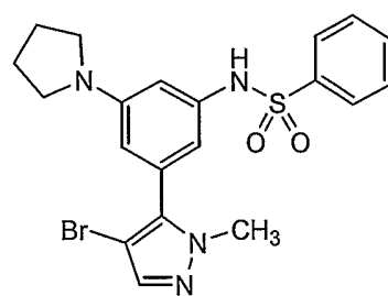
Compound 145
