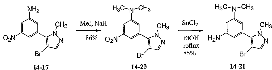
Scheme 14-4
