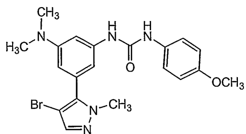
Compound 136
