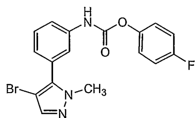
Compound 68
