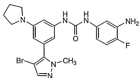
Compound 135
