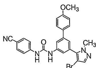
Compound 196
