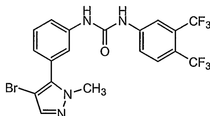
1-(3,4-Bis-trifluoromethyl-phenyl)-3-[3-(4-bromo-2-methyl-2H-pyrazol-3-yl)-phenyl]-urea
