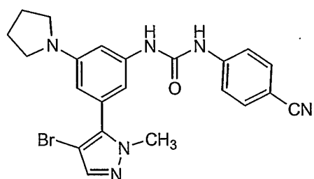
Compound 143
