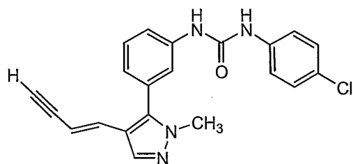
Compound 91
