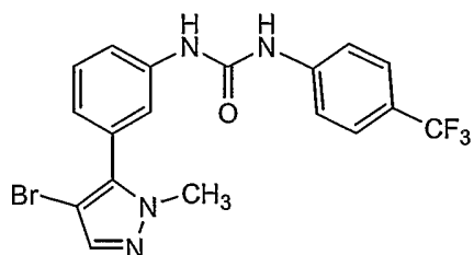
Compound 16
