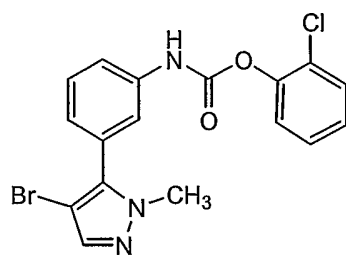
Compound 70
