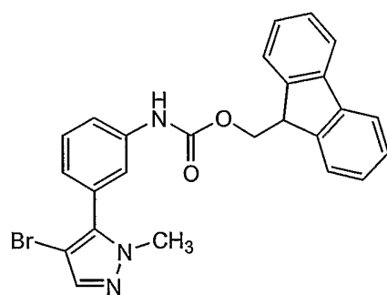
Compound 60
