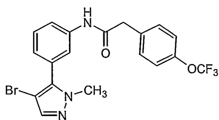
Compound 42
