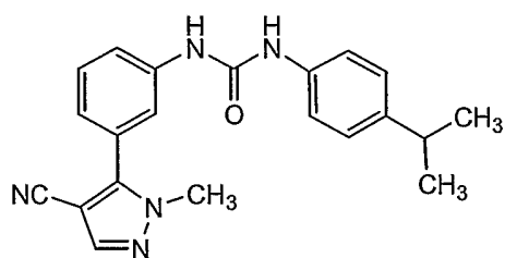
Compound 94
