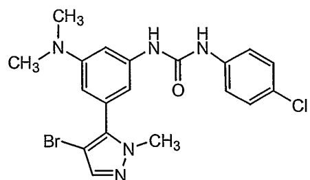
Compound 113
