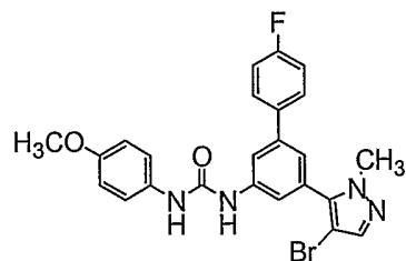
Compound 188
