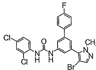
Compound 194
