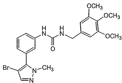
Compound 35
