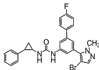
Compound 203
