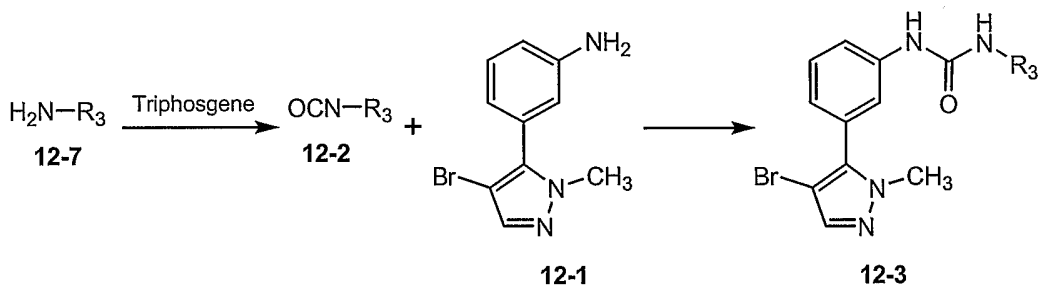
Scheme 12-3
