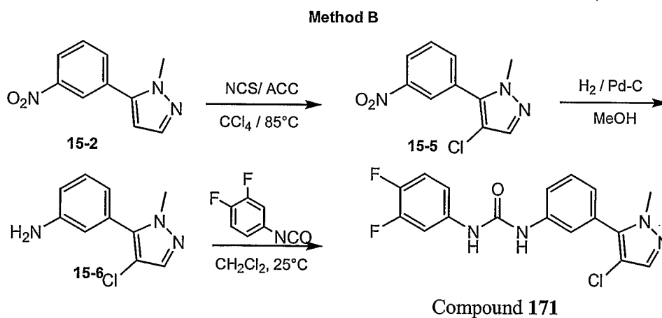
Scheme 15-3
