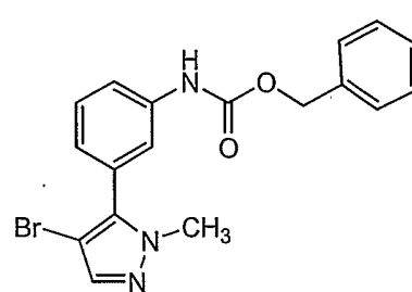
Compound 65
