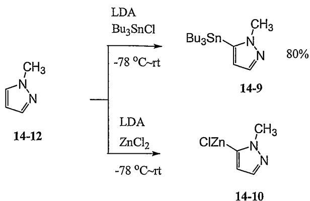
Scheme 14-1
