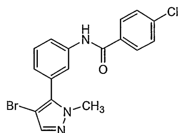
Compound 41
