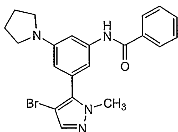
Compound 108
