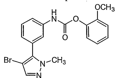
Compound 69
