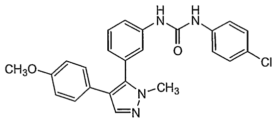
Compound 81
