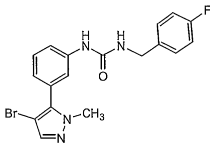
Compound 33
