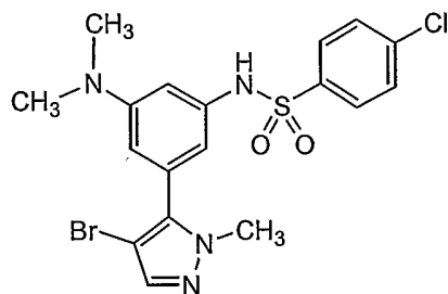
Compound 119
