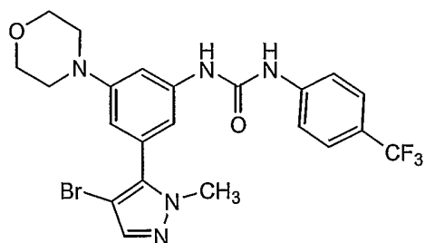
Compound 134
