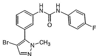
Compound 9
