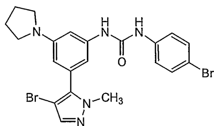
Compound 109
