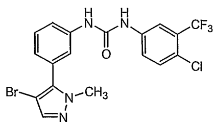
Compound 181
