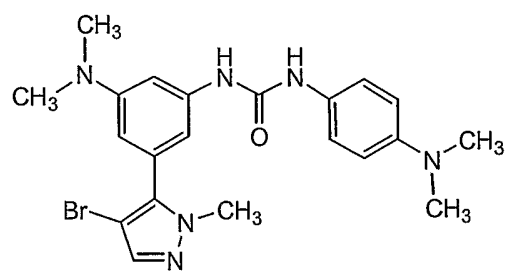
Compound 123
