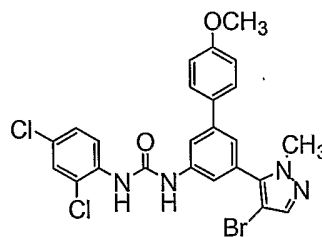
Compound 187
