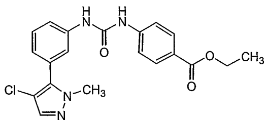
Compound 54
