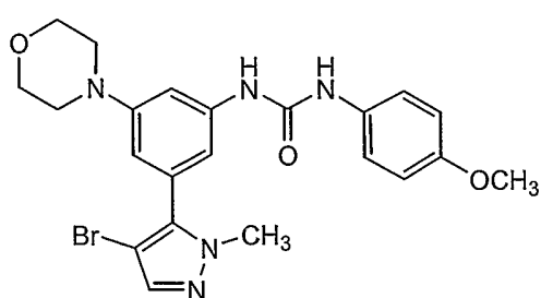
Compound 146
