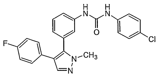
Compound 83
