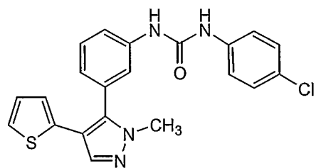
Compound 85
