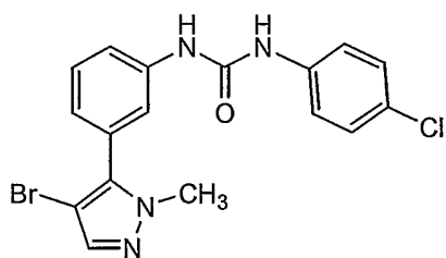
Compound 8
