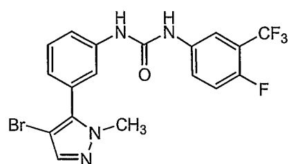
Compound 170
