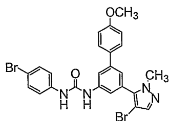
Compound 200
