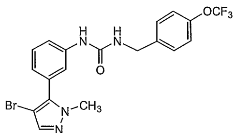
Compound 10
