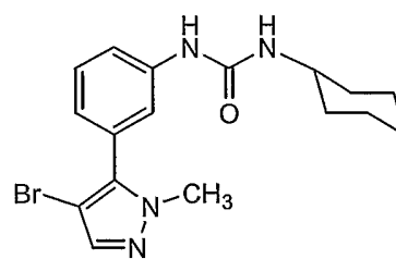
Compound 31
