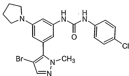
Compound 141
