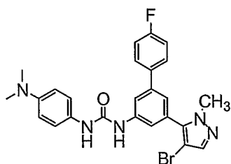
Compound 189
