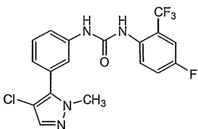
Compound 179
