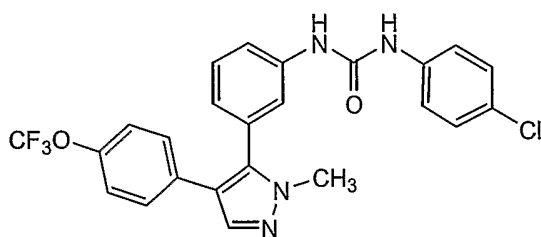
Compound 84
