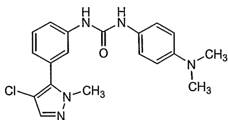
Compound 53
