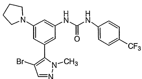
Compound 160
