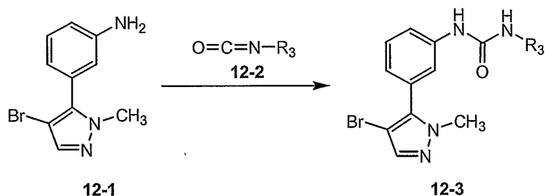
Scheme 12-1
