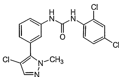
Compound 50
