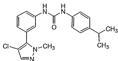
Compound 56
