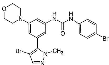
Compound 142
