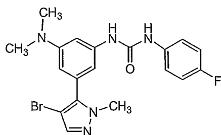
Compound 129
