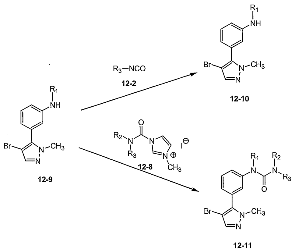
Scheme 12-5
