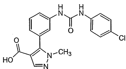
Compound 86
