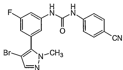
Compound 102
