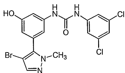
Compound 150
