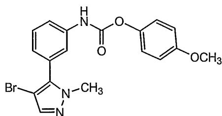
Compound 1
