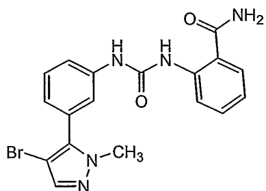
Compound 28
