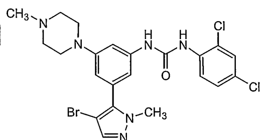
Compound 133
