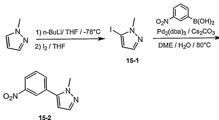
Scheme 15-1
