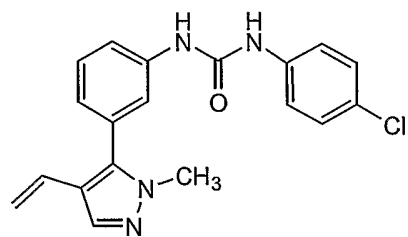
Compound 77
