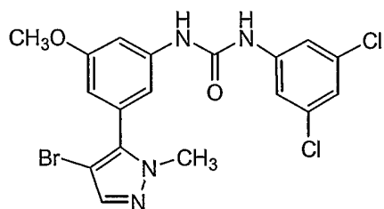
Compound 156
