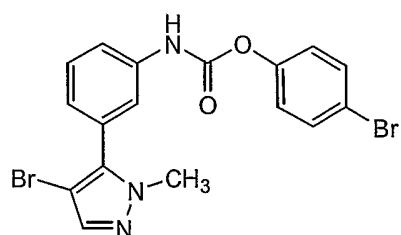
Compound 67
