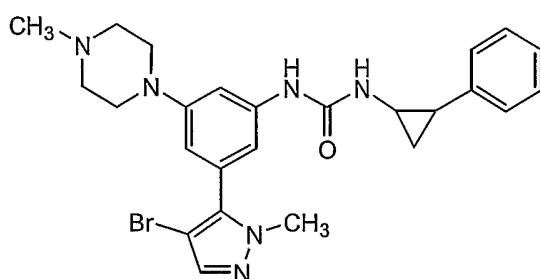
Compound 132
