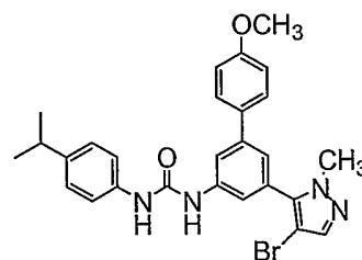
Compound 201
