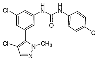
Compound 49
