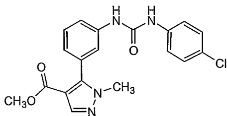
Compound 74
