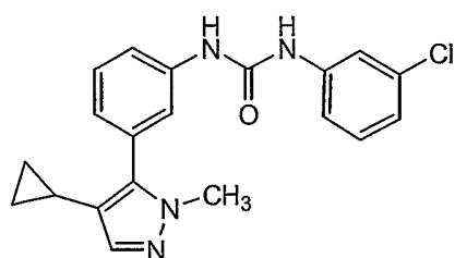
Compound 88
