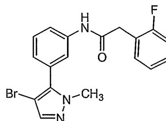
Compound 45
