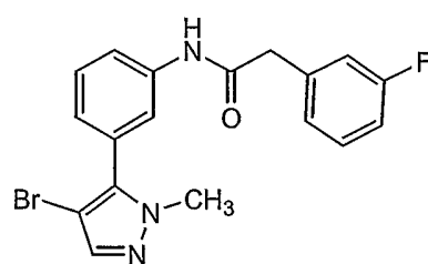
Compound 43
