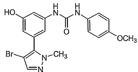
Compound 161
