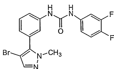
Compound 165
