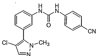
Compound 52
