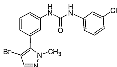
Compound 17
