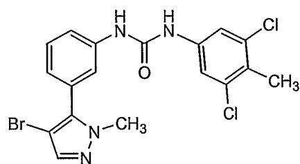
Compound 25
