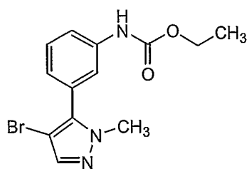
Compound 58
