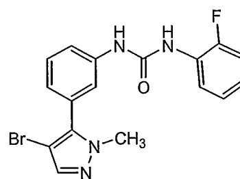
Compound 27
