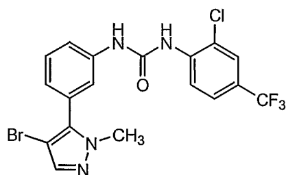
1-[3-(4-Bromo-2-methyl-2H-pyrazol-3-yl)-phenyl]-3-(2-chloro-4-trifluoromethyl-phenyl)-urea
