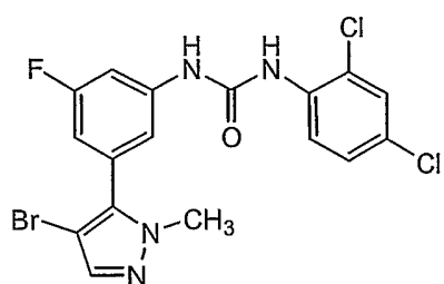
Compound 104
