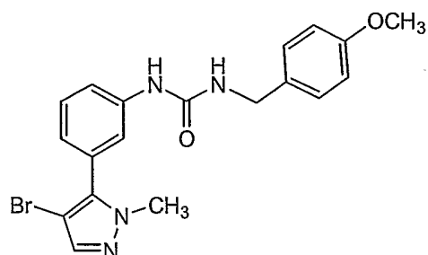
Compound 37
