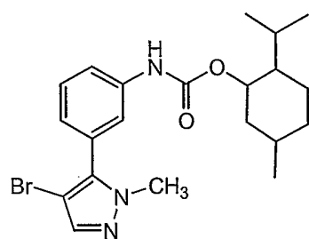
Compound 64
