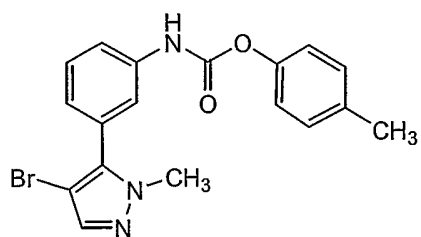
Compound 62
