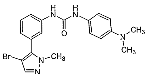
Compound 24
