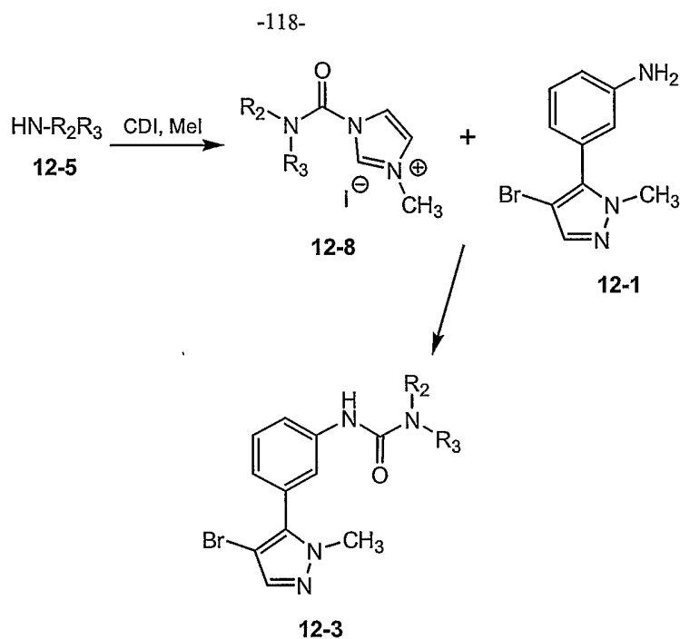
Scheme 12-4
