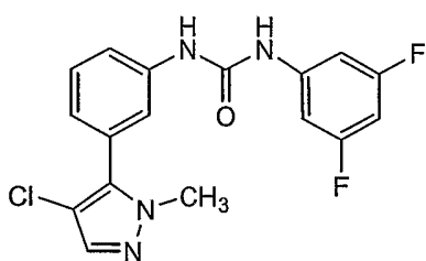
Compound 175
