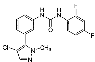
Compound 177
