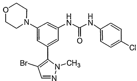
Compound 121
