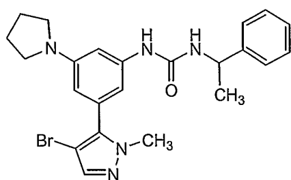
Compound 106
