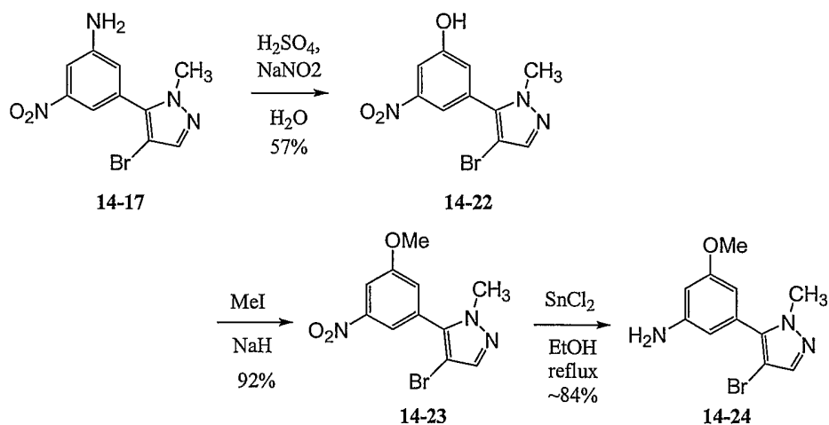
Scheme 14-5
