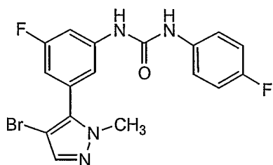
Compound 100
