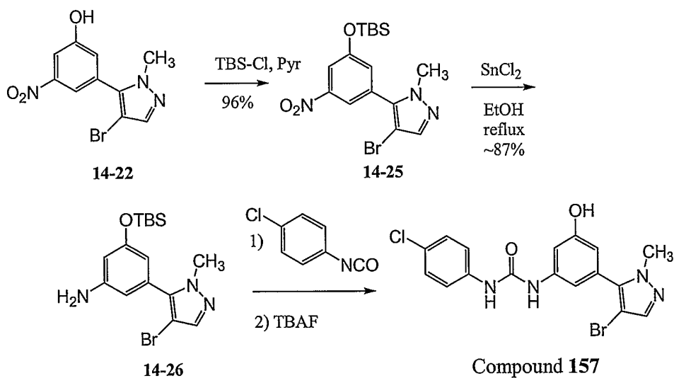
Scheme 14-6
