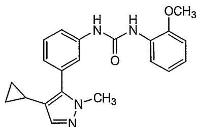
Compound 89
