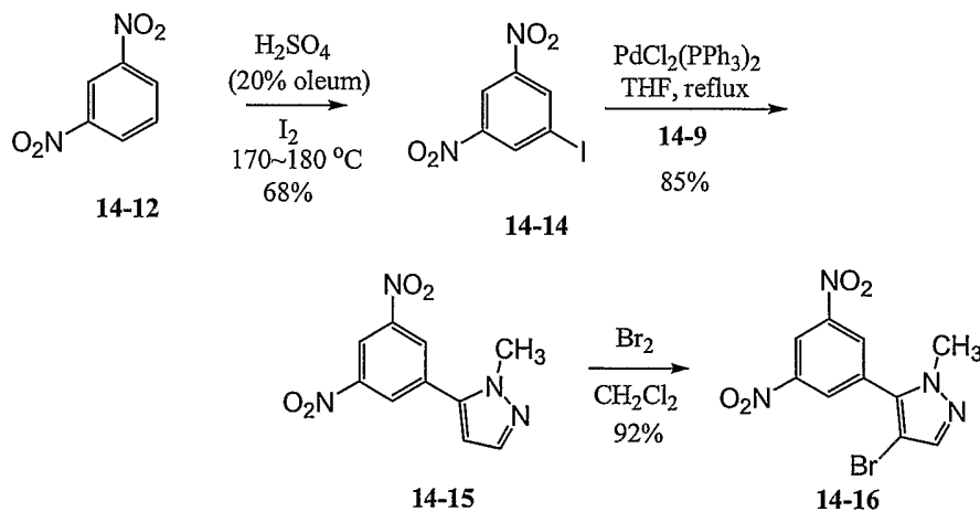
Scheme 14-2
