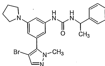
Compound 139
