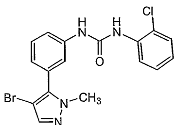
Compound 18
