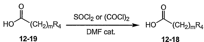
Scheme 12-14
