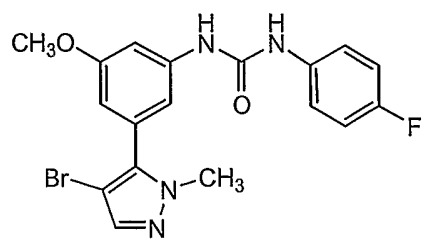
Compound 149
