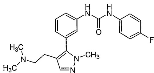
Compound 76
