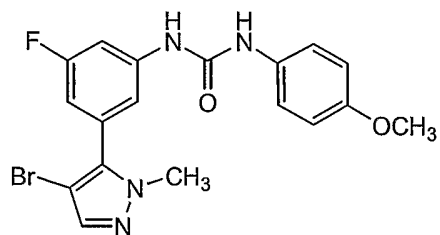
Compound 101
