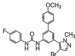
Compound 192
