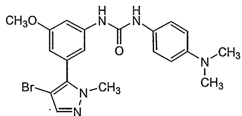
Compound 153
