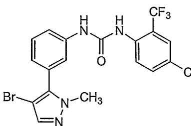
Compound 180
