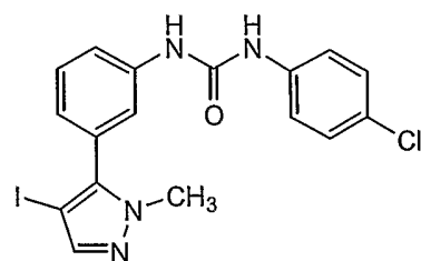
Compound 57
