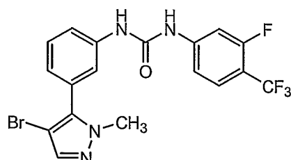
1-[3-(4-Bromo-2-methyl-2H-pyrazol-3-yl)-phenyl]-3-(3-fluoro-4-trifluoromethyl-phenyl)-urea
