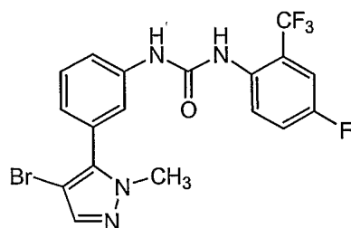
Compound 169
