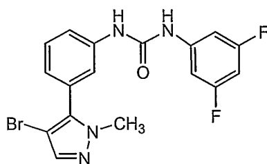
Compound 167
