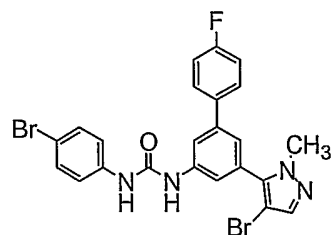
Compound 197
