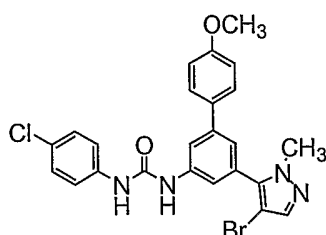
Compound 191
