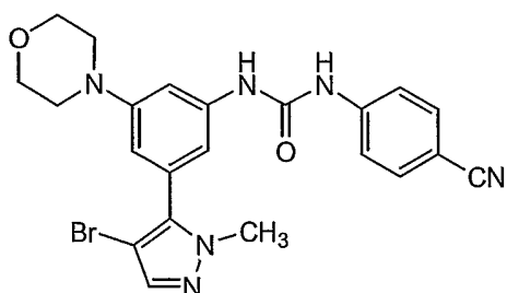
Compound 128
