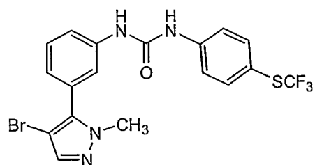
Compound 26
