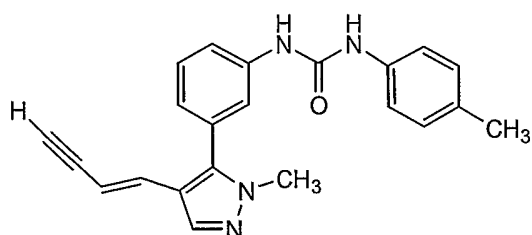
Compound 92
