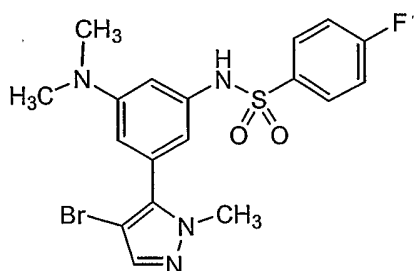
Compound 144
