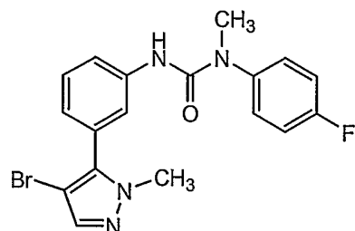
3-[3-(4-Bromo-2-methyl-2H-pyrazol-3-yl)-phenyl]-1-(4-fluorophenyl)-1-methyl-urea
