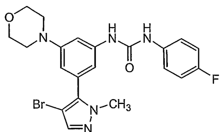
Compound 120
