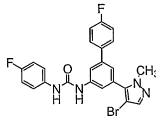
Compound 204
