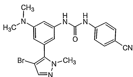
Compound 138
