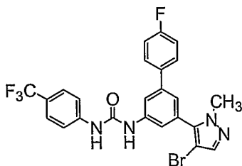
Compound 190
