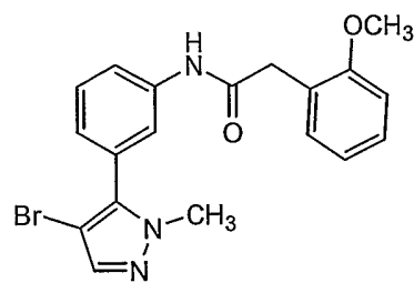
Compound 47
