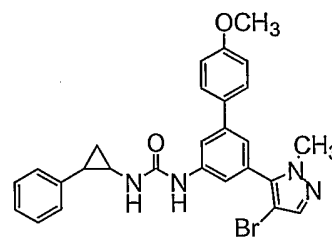
Compound 202
