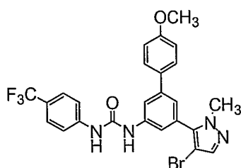
Compound 186
