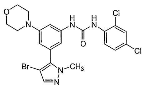
Compound 107
