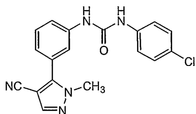
Compound 93
