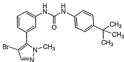
Compound 23
