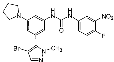
Compound 137
