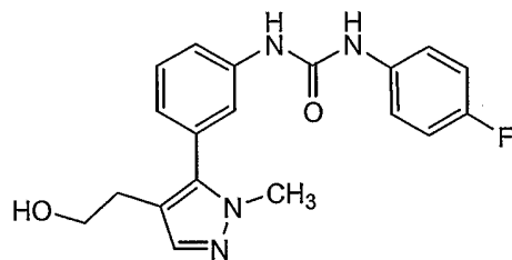
Compound 75
