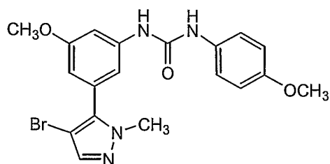
Compound 162
