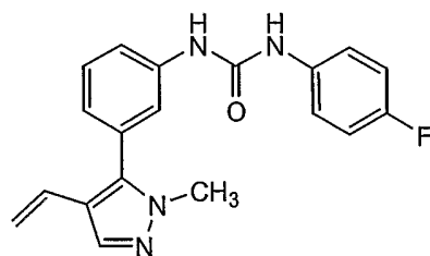
Compound 79
