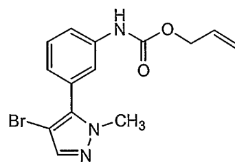
Compound 61
