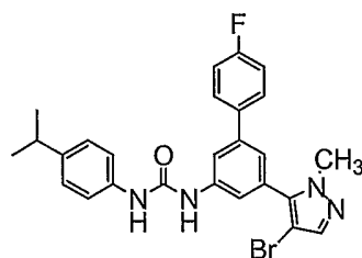
Compound 195
