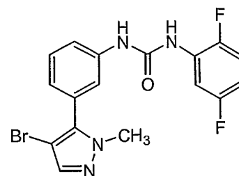
Compound 172
