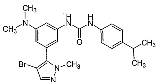
Compound 130
