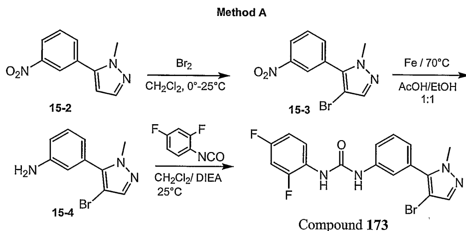
Scheme 15-2
