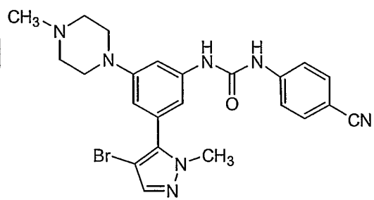
Compound 127
