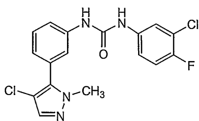
Compound 176
