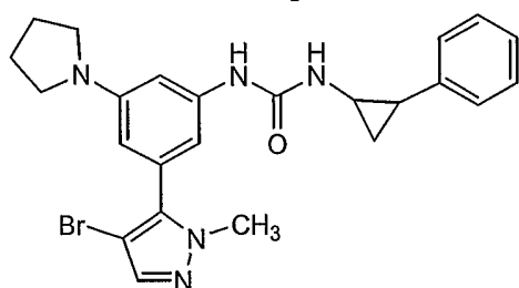
Compound 140
