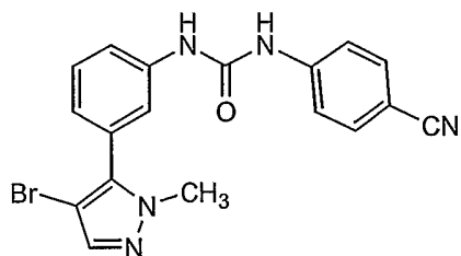
Compound 29
