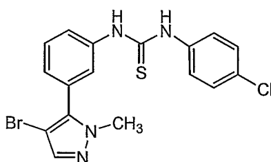
Compound 164
