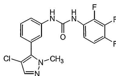
Compound 178
