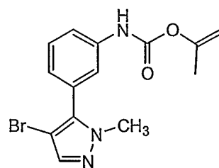
Compound 71
