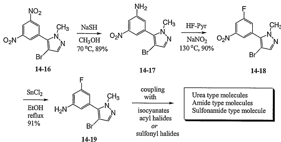
Scheme 14-3
