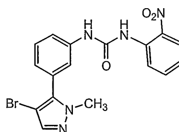
Compound 13
