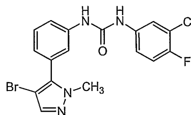
Compound 168
