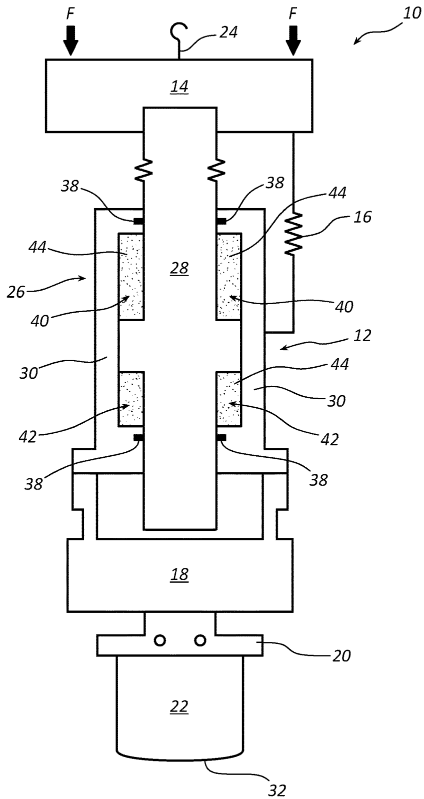
FIG. 3 (Prior Art)
