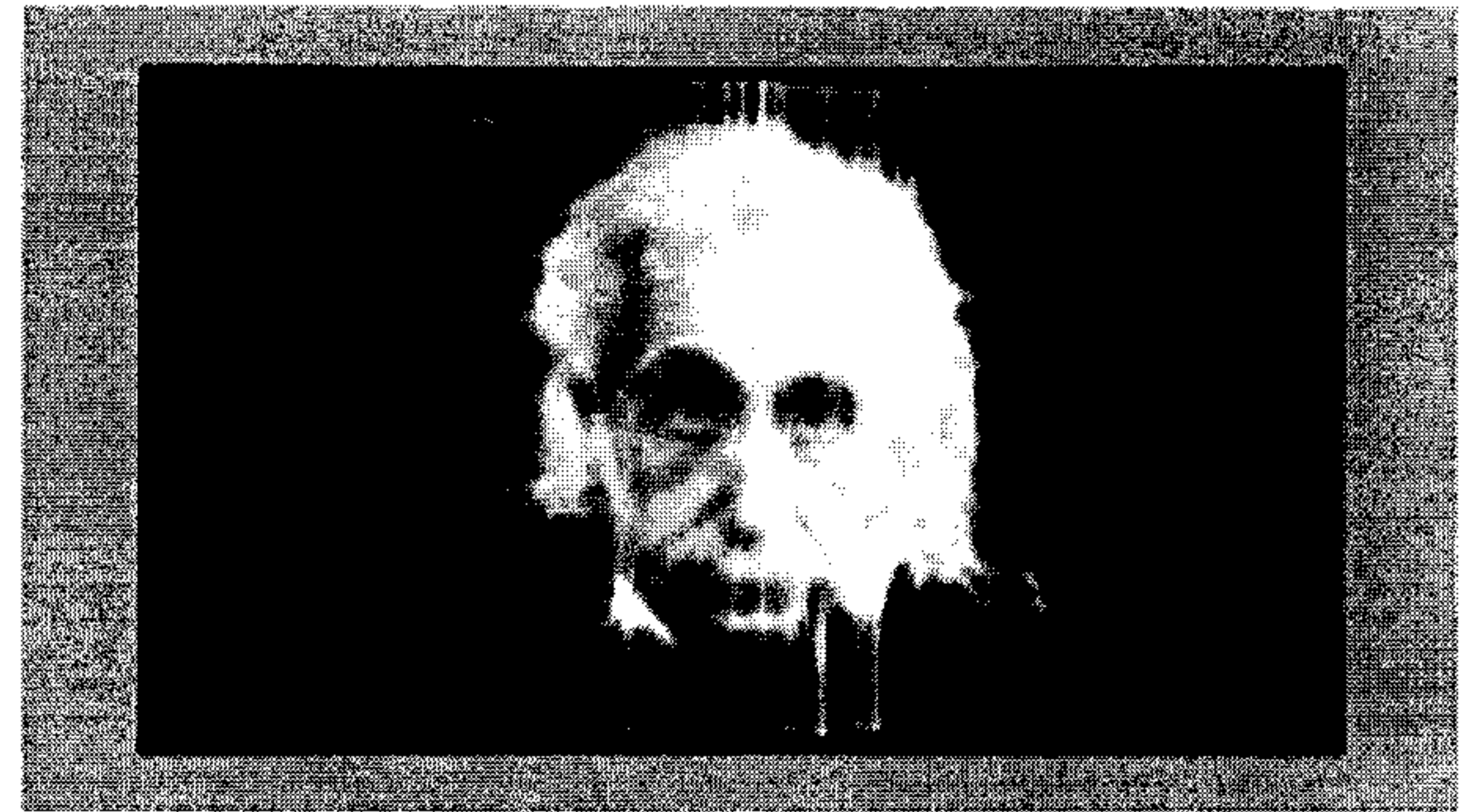
FIG. 26B \beta = 1.0
