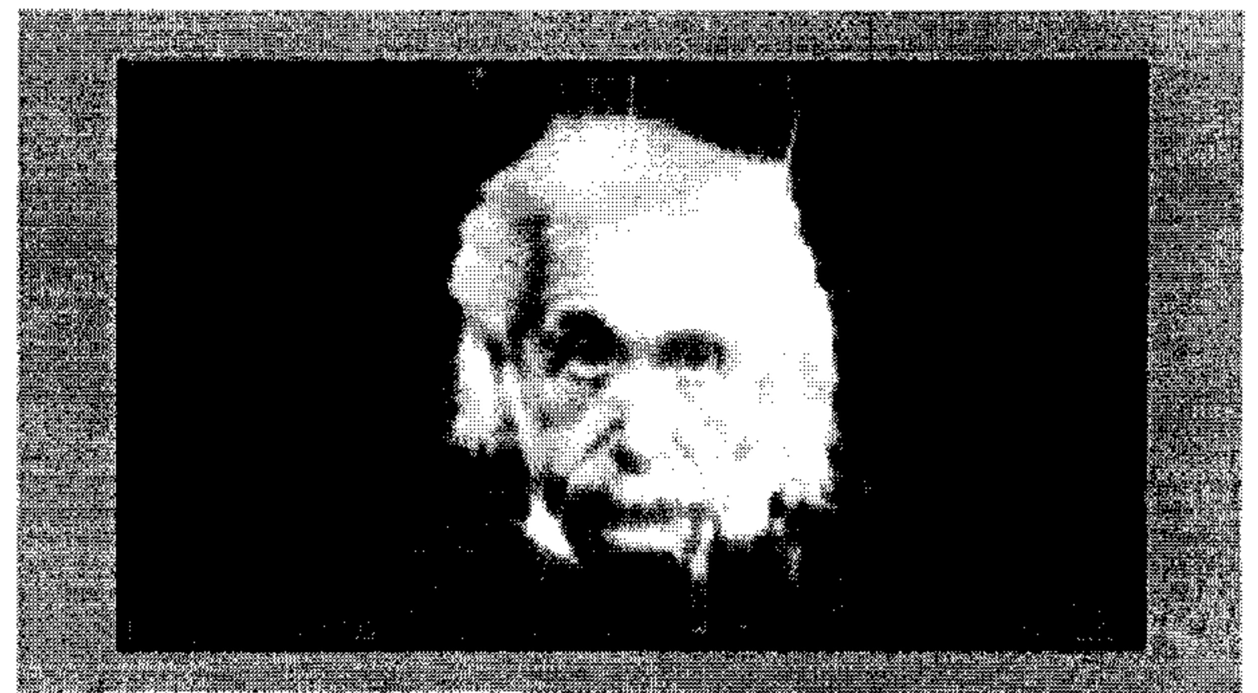
FIG. 26D \beta = 100.0
