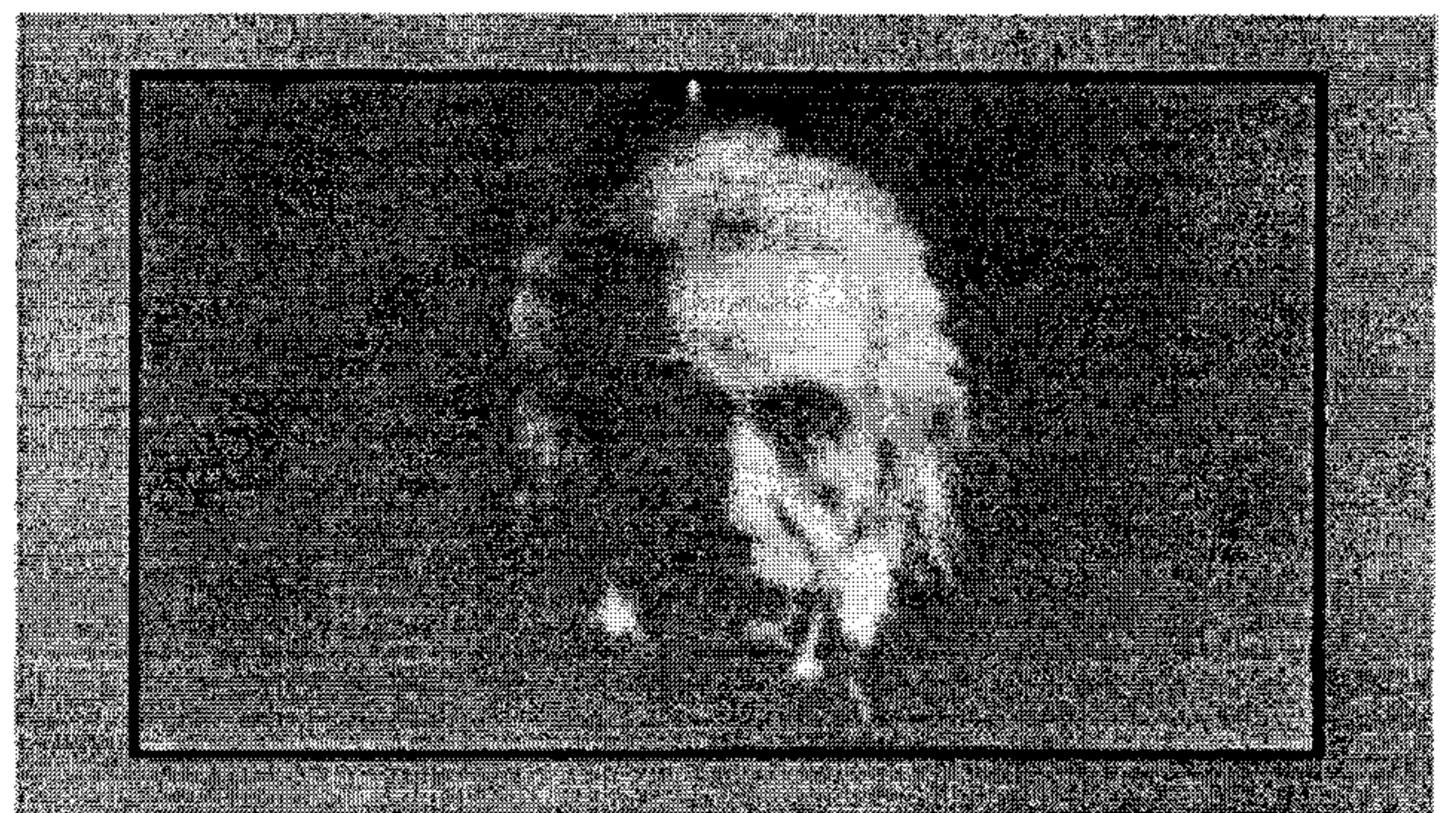
FIG. 28D \epsilon = 1.0
