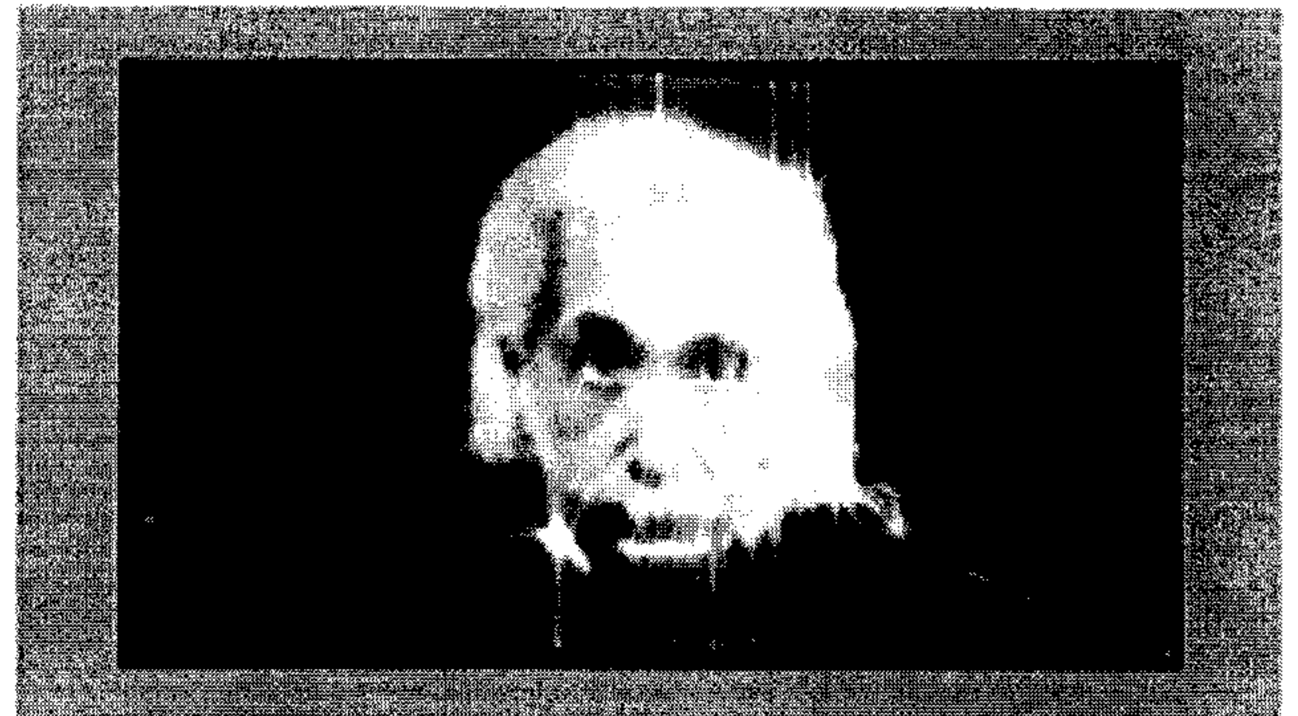
FIG. 28B \epsilon = 0.01
