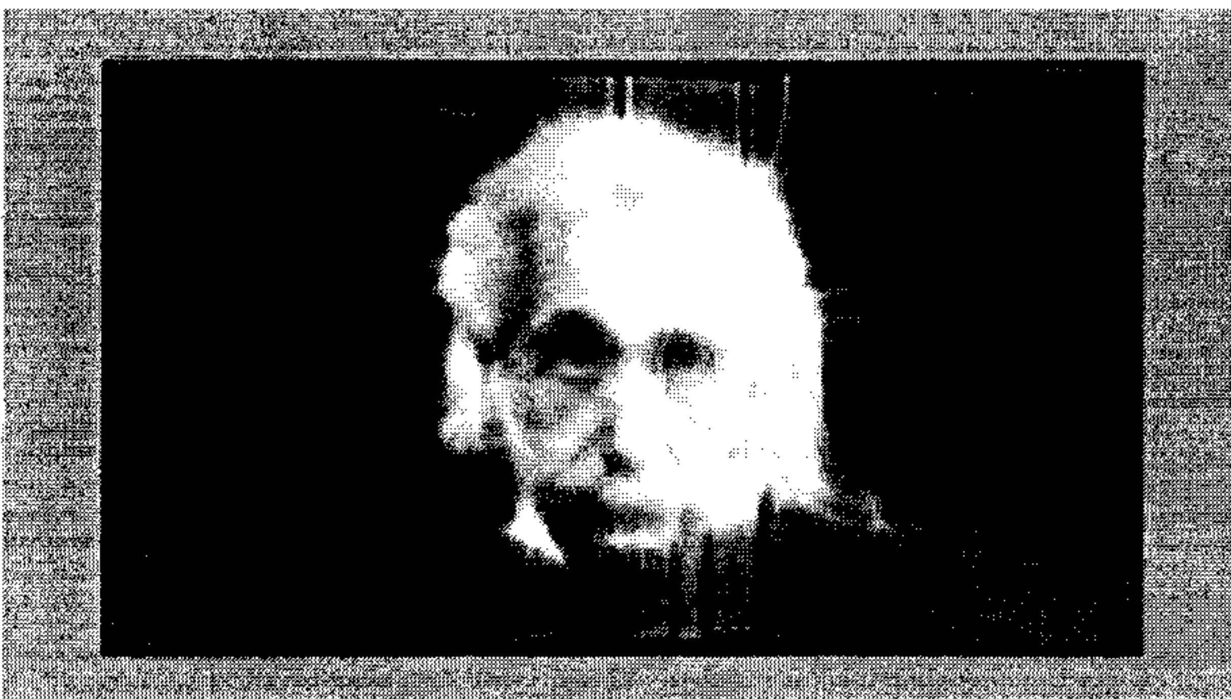
FIG. 26C \beta = 10.0
