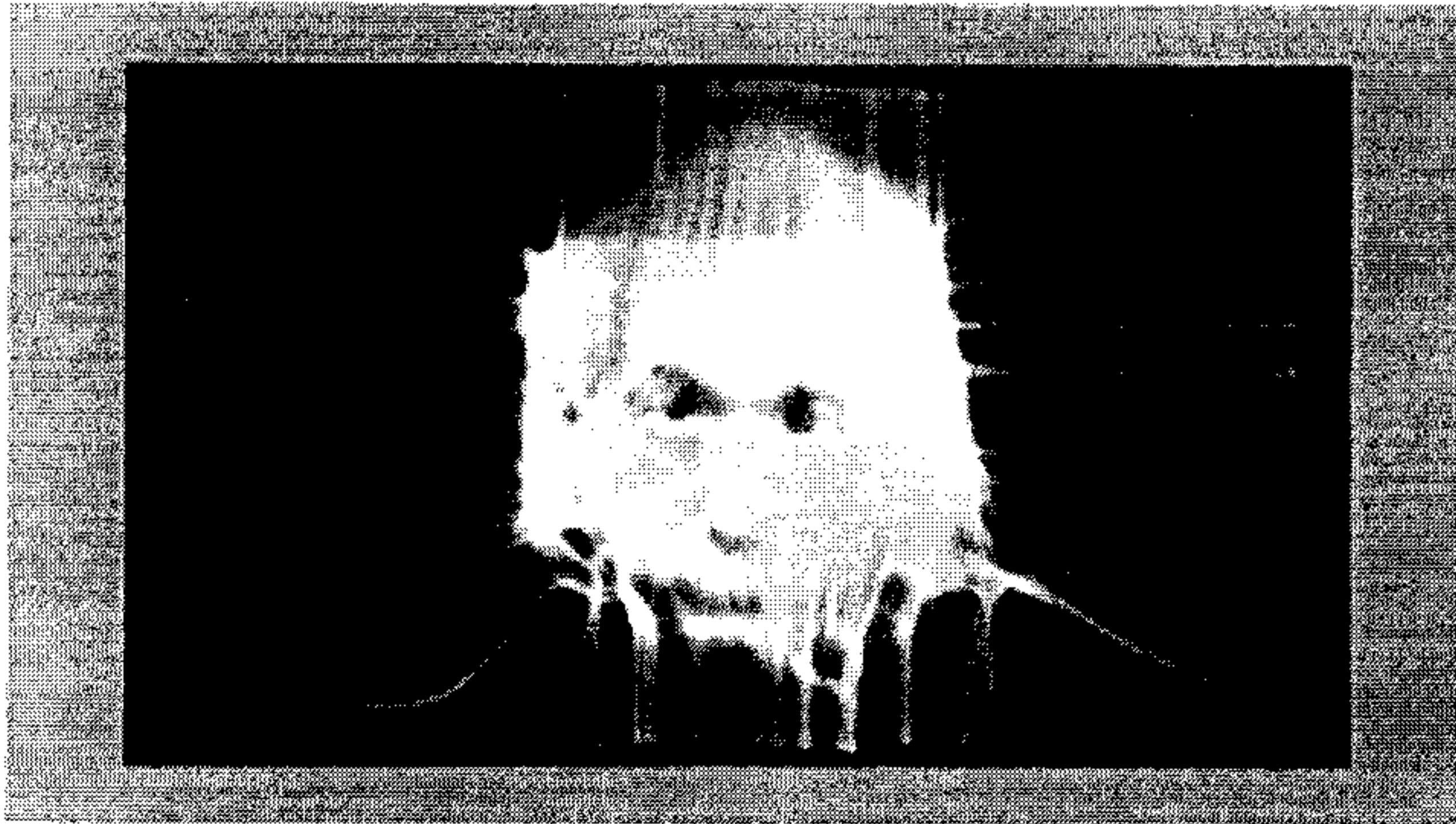
FIG. 28A \epsilon = 0.001
