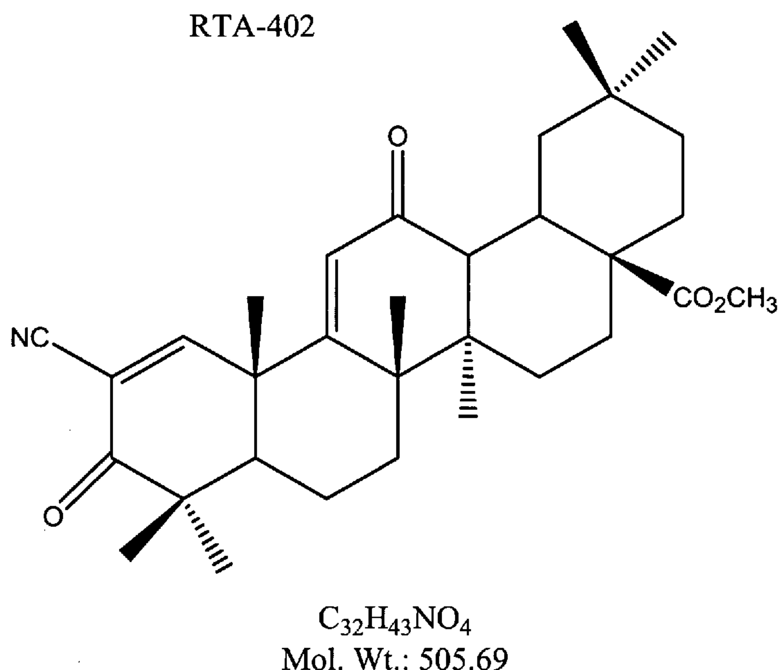
Figure 1 - Chemical structure of CDDO methyl ester
