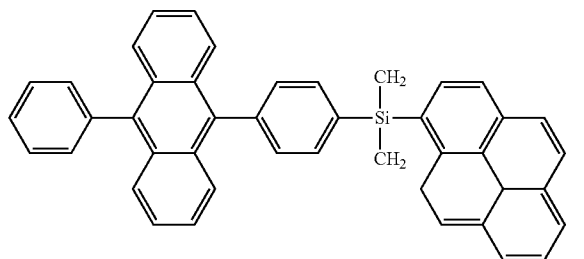
Compound 22
