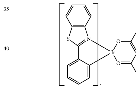
Ir(BT) 2 (acac)
