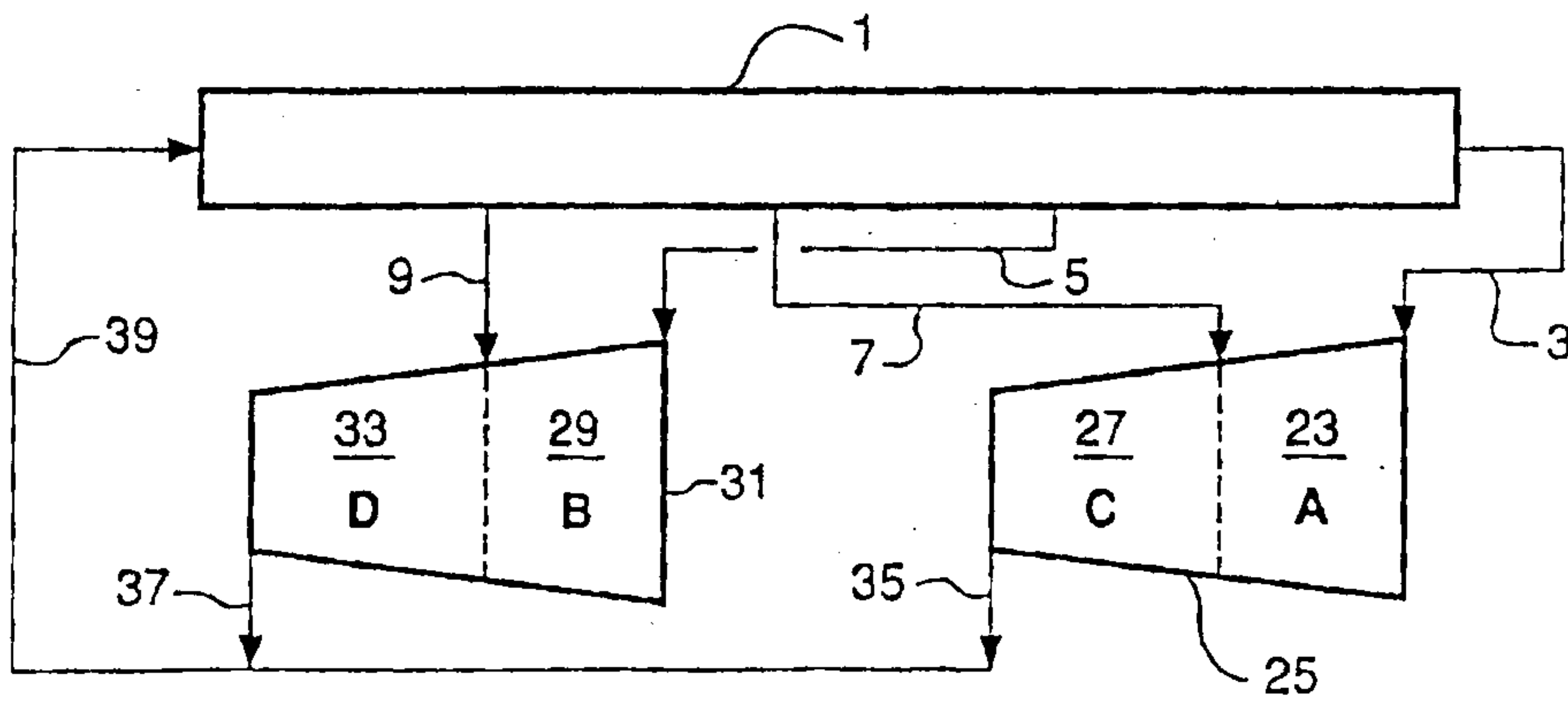
FIG. 2 (PRIOR ART)
