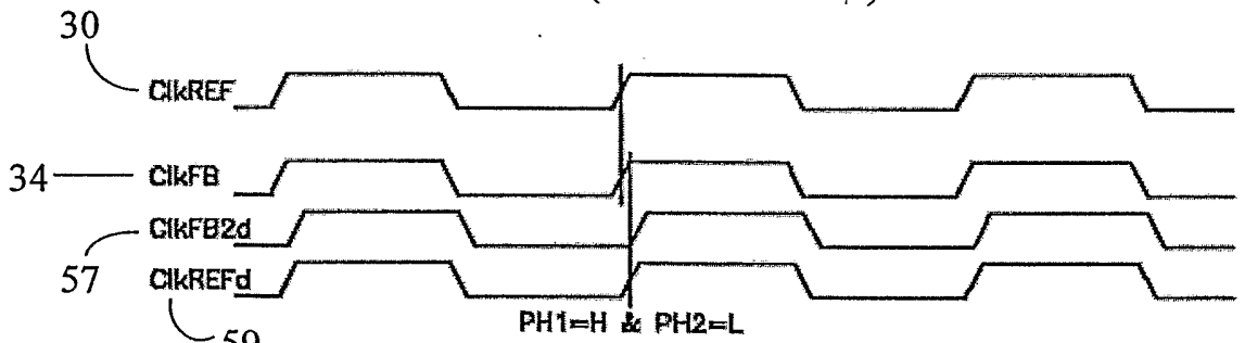
FIG. 7B (PRIOR ART)
