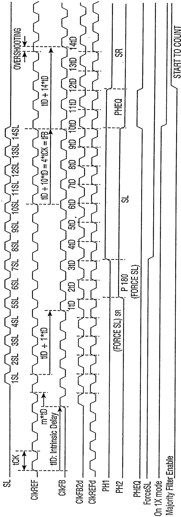
Prior Art Fig. 12
