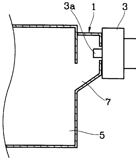
FIG.1 (PRIOR ART)
