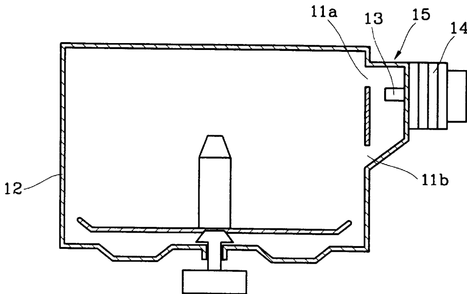
FIG.4 (PRIOR ART)
