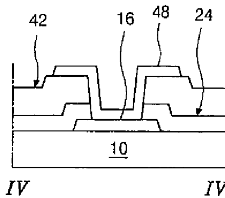
FIG. 4D (Related Art)
