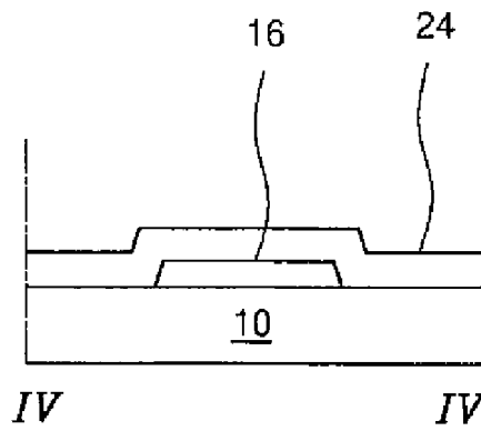
FIG. 4A (Related Art)
