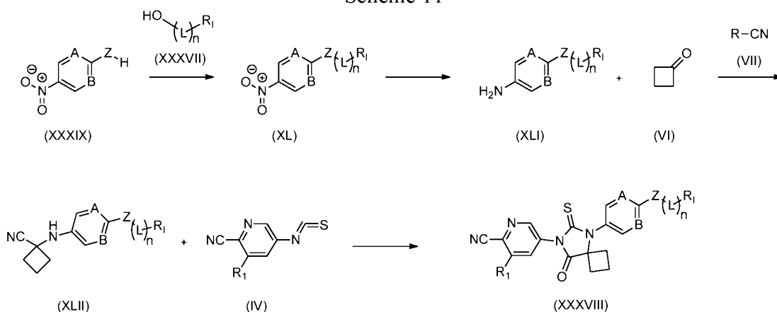
Scheme 11
