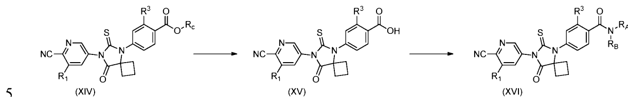
Scheme 5
