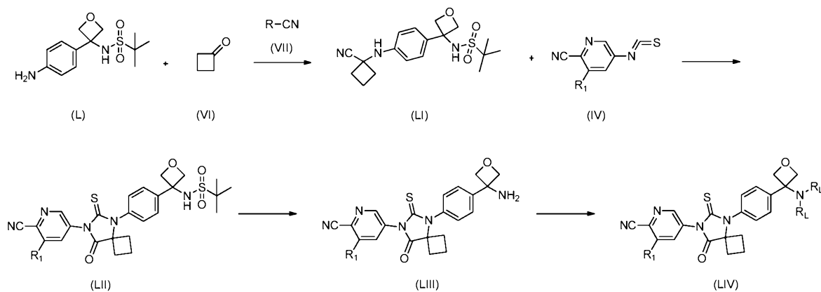
Scheme 14
