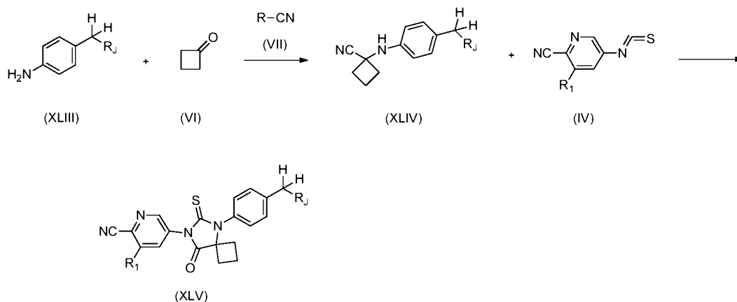
Scheme 12
