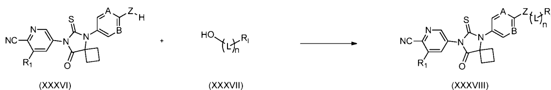
Scheme 10
