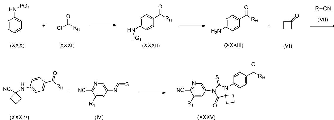
Scheme 9
