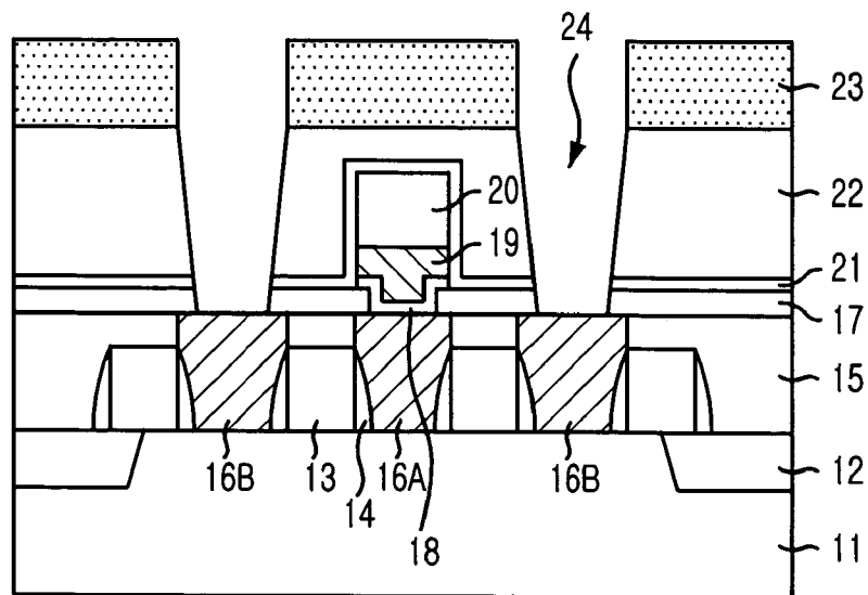
FIG. 1C (PRIOR ART)
