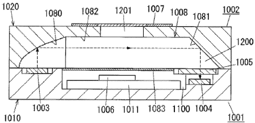
FIG. 45 PRIOR ART
