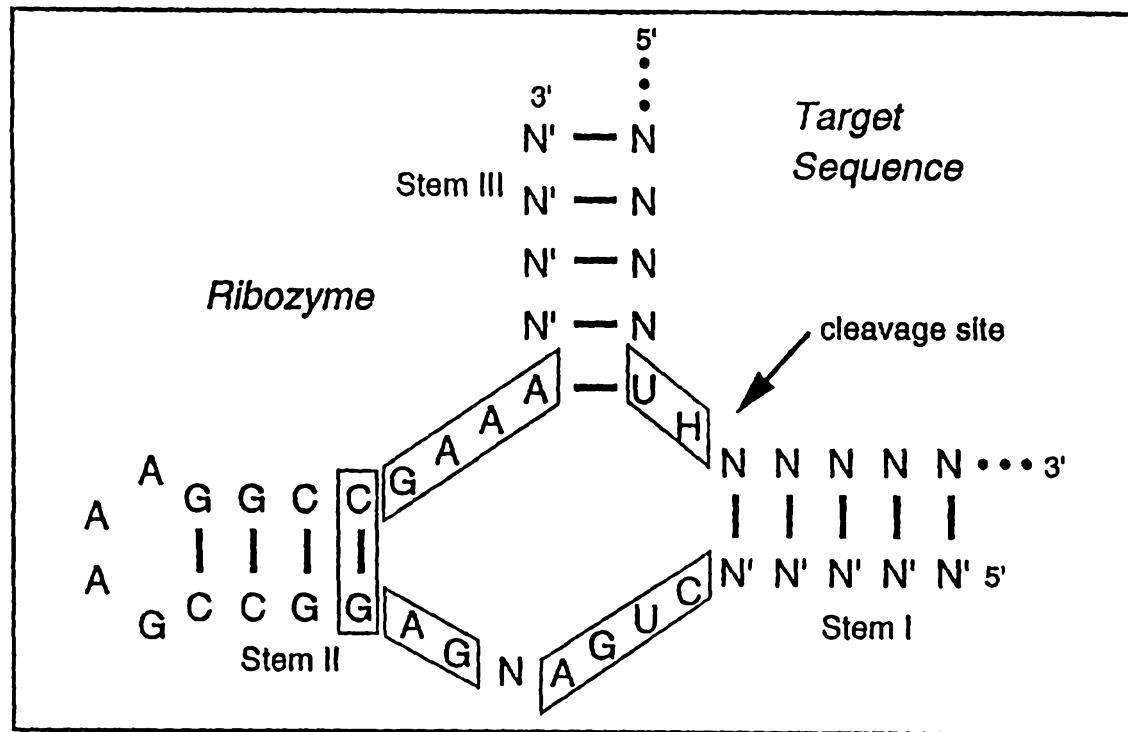
Figure 1: Hammerhead Ribozyme
