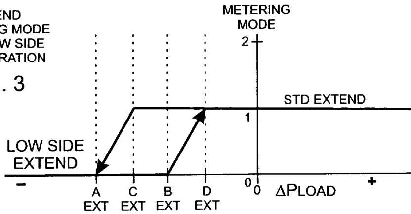
EXTEND METERING MODE WITH HIGH SIDE REGENERATION FIG. 5
