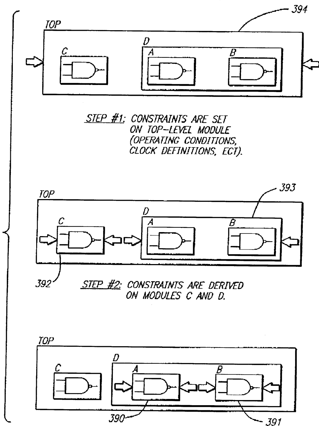
FIG. 16 TOP-DOWN CHARACTERIZATION
