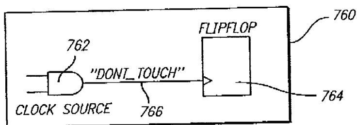
FIG. 41C CLOCK SOURCE RETREIVED THROUGH USING THE CONNECTED NET. RETRIEVING NAMES OF NEW SOURCE PINS.
