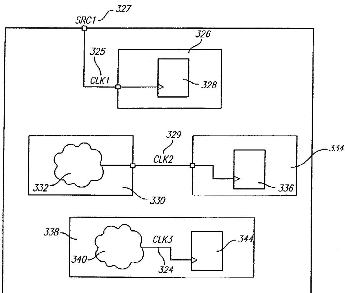
FIG. 39 EXTERNAL AND INTERNAL CLOCKS
