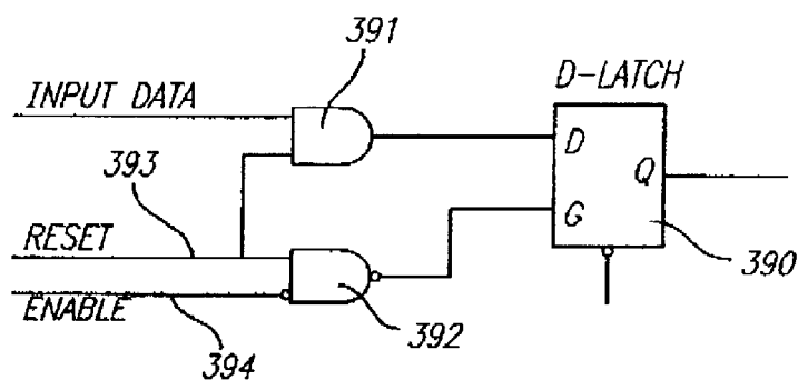
FIG. 37 FAILING IMPLEMENTATION OF A LATCH WITH CLEAR
