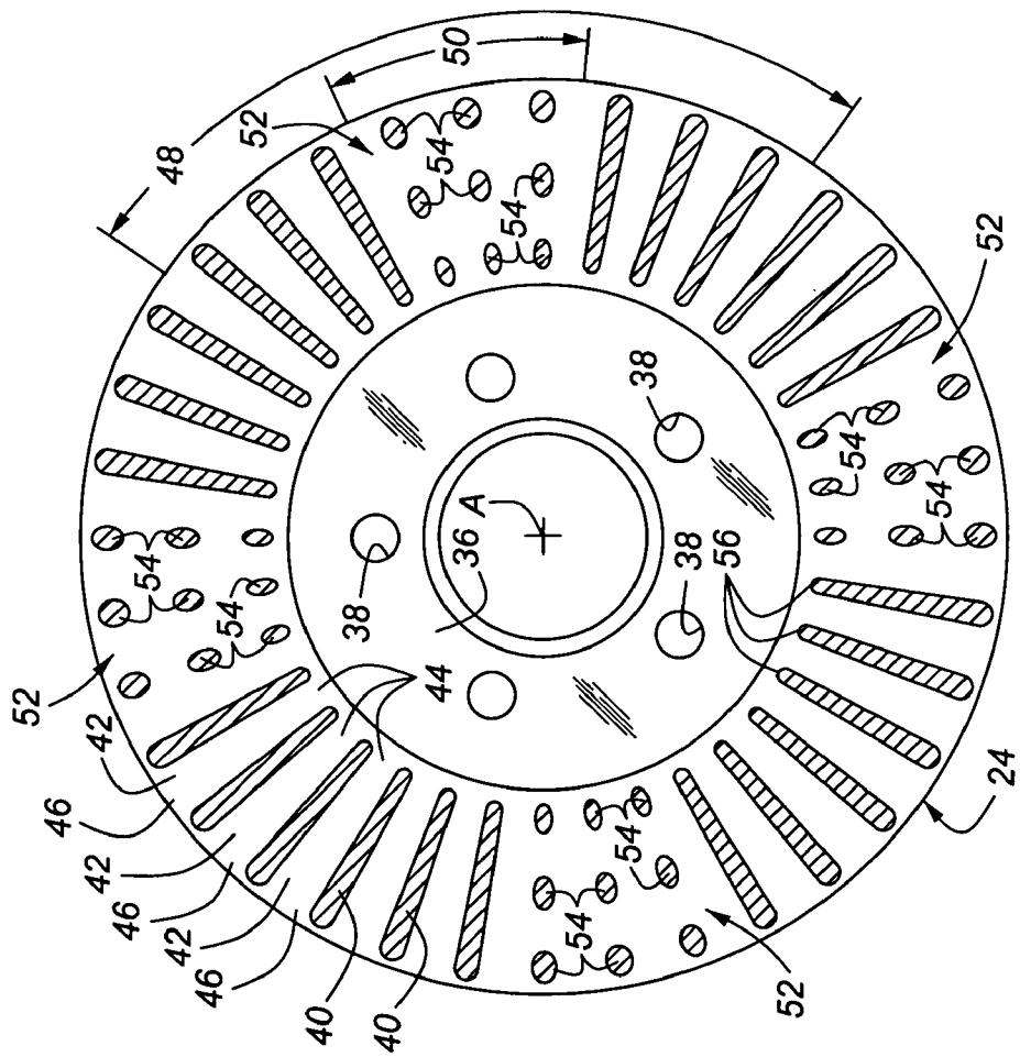
Figure 11A
