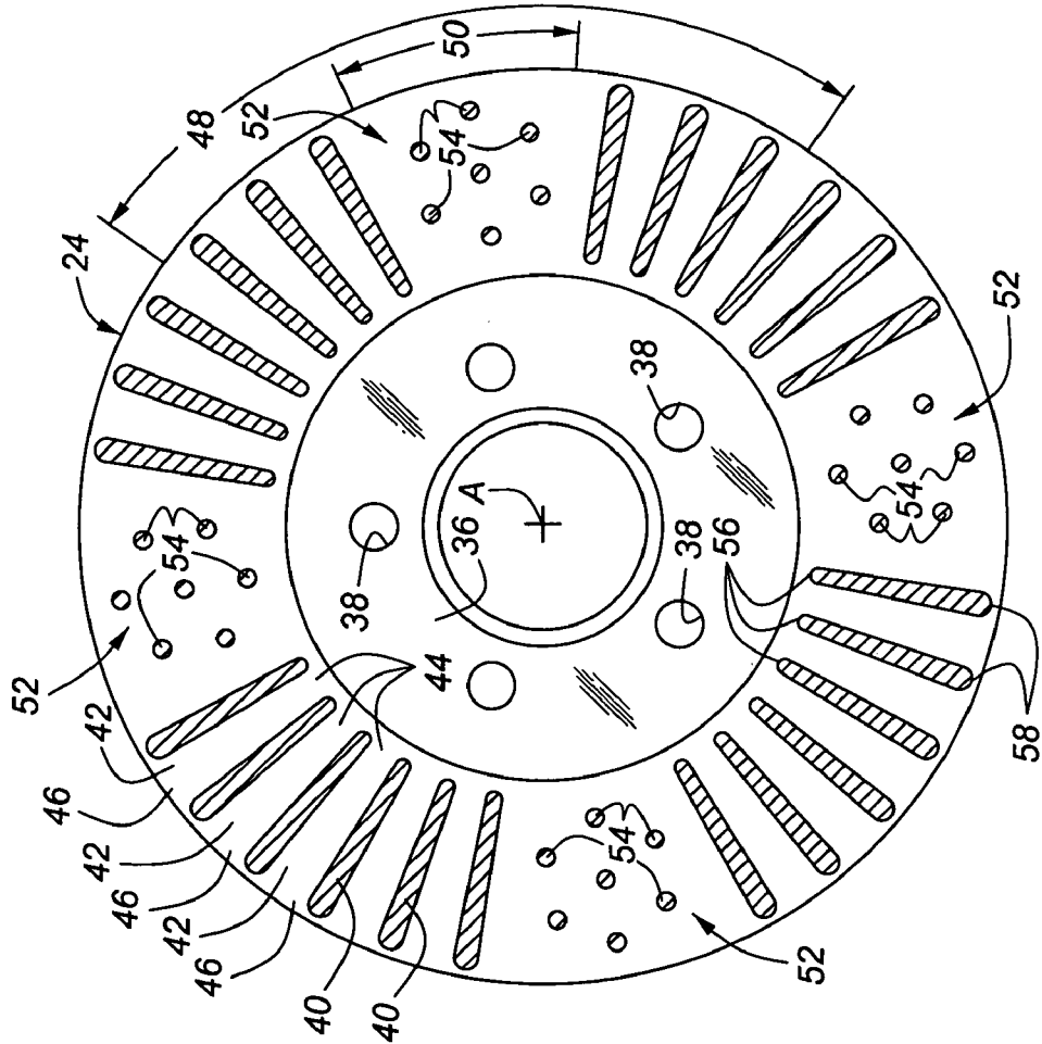
Figure 14A
