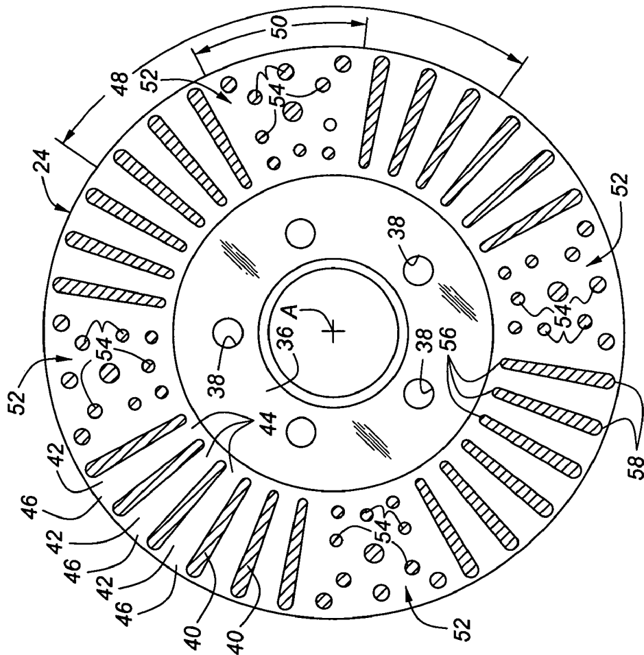
Figure 19A
