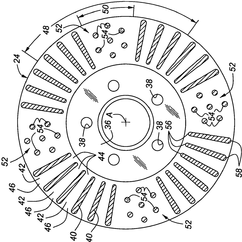
Figure 15A
