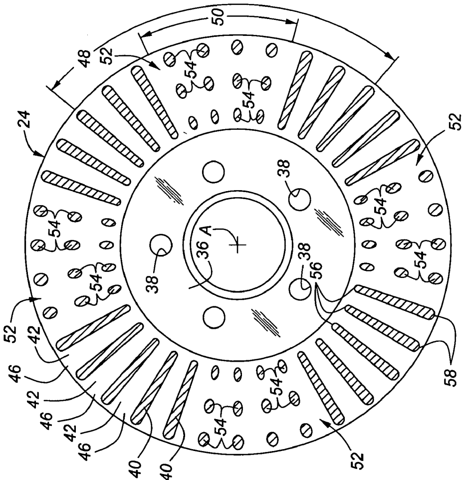
Figure 13A
