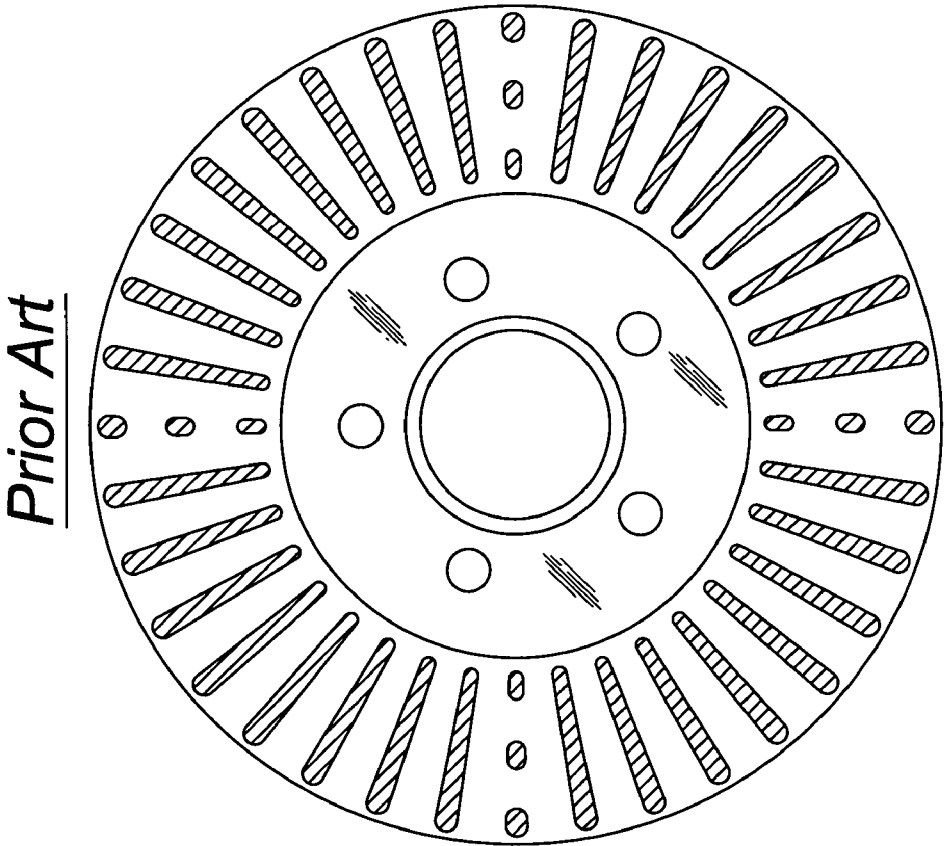
Figure 6A
