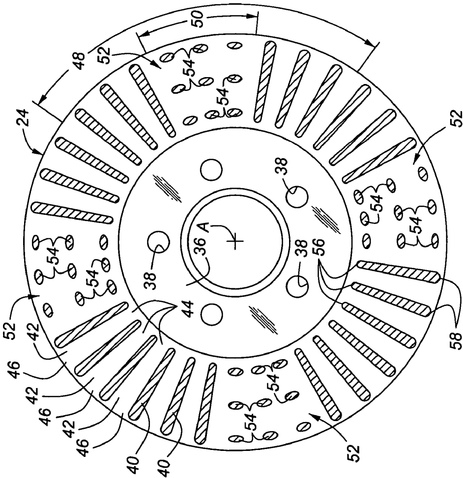
Figure 12A
