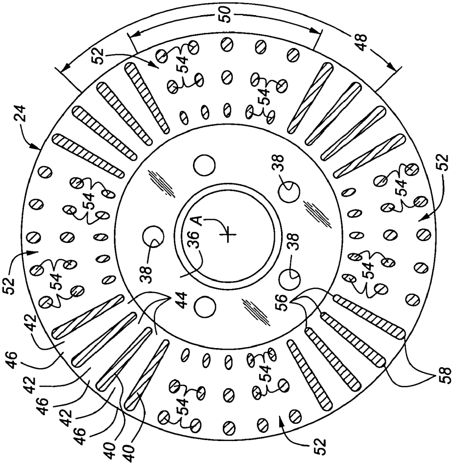
Figure 21A
