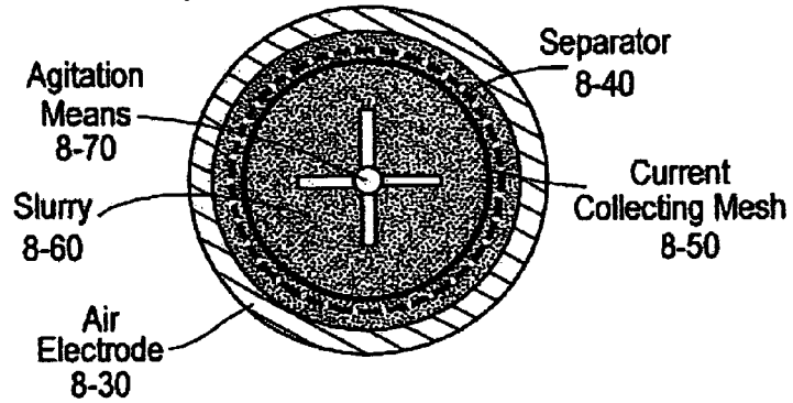
Top View Schematic
