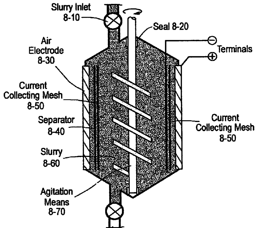
Fig.8 Side View Schematic
