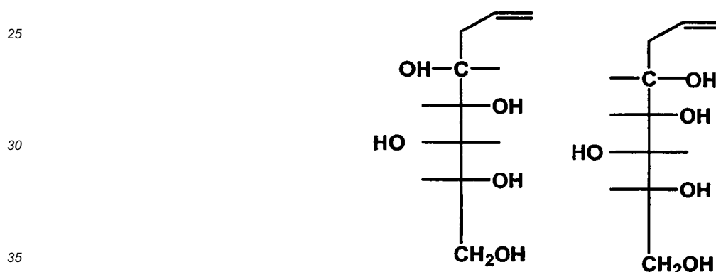
1,2,3-trideoxy-D-ido-octenitol
