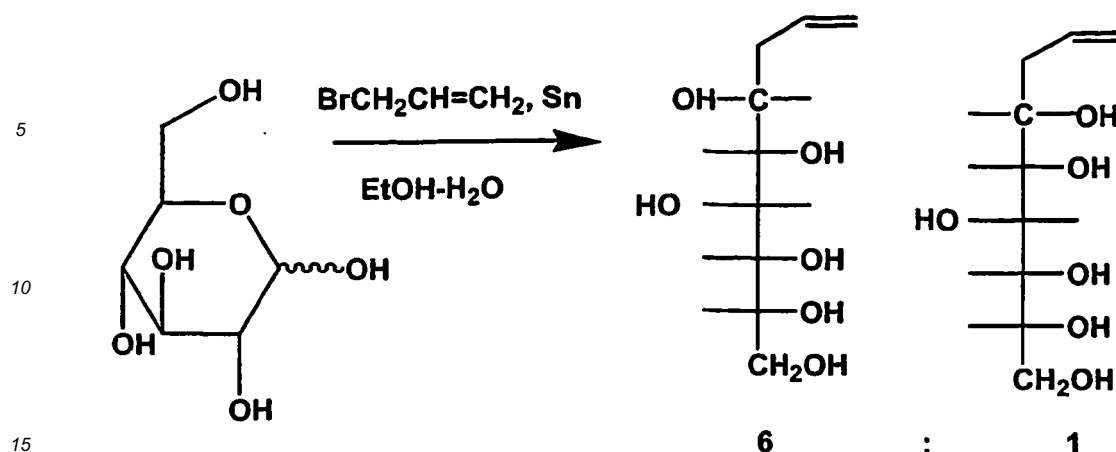
1,2,3-trideoxy-D-glycero-D-ido-nonenitol
