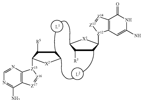
Formula Ib
