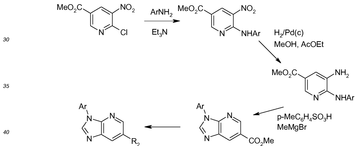
Scheme 9B
