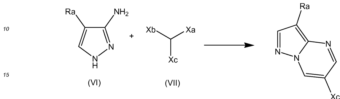
Scheme 5A
