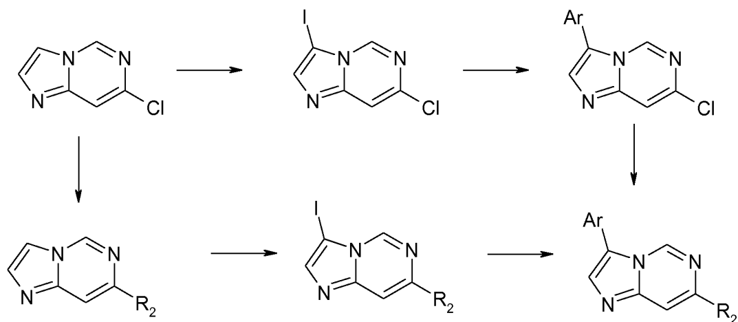
Scheme 14
