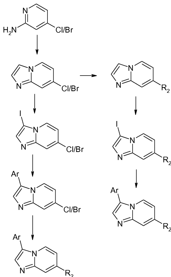
Scheme 2
