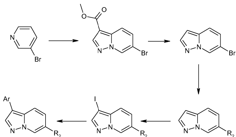
Scheme 7
