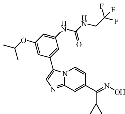
Compound 1-66 (E-isomer)
