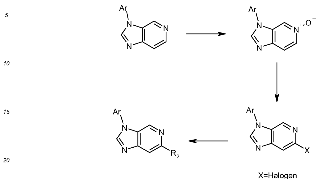
Scheme 11
