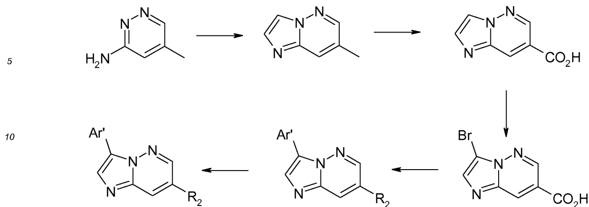
Scheme 19
