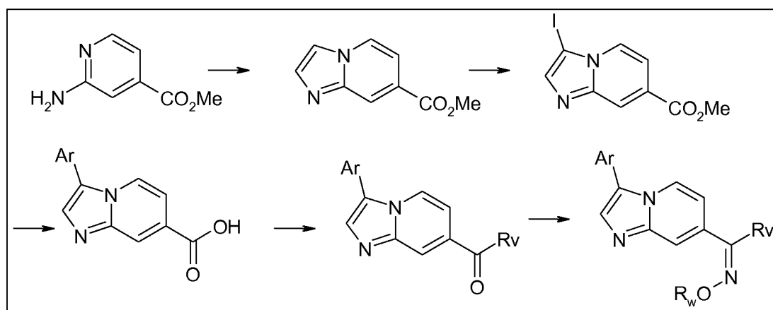
Scheme 1B
