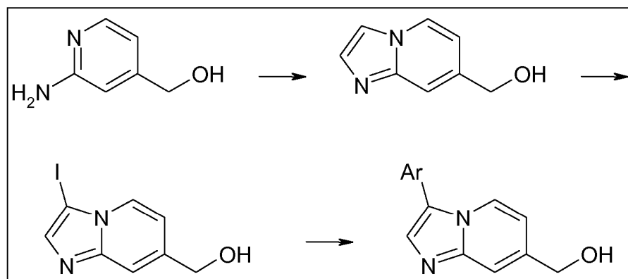
Scheme 1C
