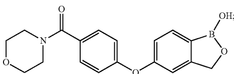
5-(3,4-Dicyanophenoxy)-1,3-dihydro-1-hydroxy-2,1-benzoxaborole
