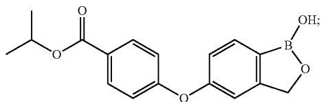
4-(1-Hydroxy-1,3-dihydro-benzo[c][1,2]oxaborol-5-yloxy)-benzoic acid isopropyl ester
