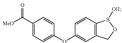
4-(1-Hydroxy-1,3-dihydro-benzo[c][1,2]oxaborol-5-yloxy)-benzoic acid ethyl ester
