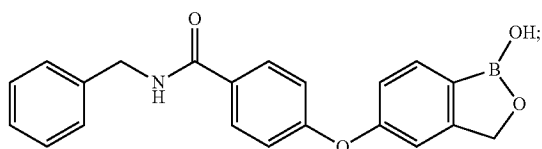
N-Benzyl-4-(1-hydroxy-1,3-dihydro-benzo[c][1,2]oxaborol-5-yloxy)-benzamide
