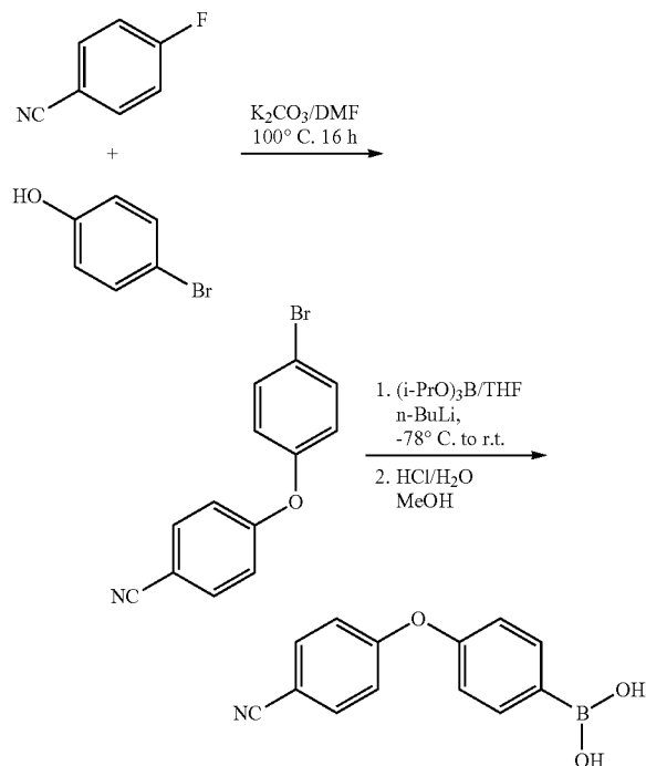
(a) 4-(4-cyanophenyl)(4-bromophenyl)ether
