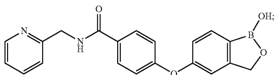
4-(1-Hydroxy-1,3-dihydro-benzo[c][1,2]oxaborol-5-yloxy)-N-pyridin-2-ylmethyl-benzamide
