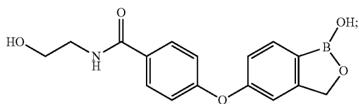
4-(1-Hydroxy-1,3-dihydro-benzo[c][1,2]oxaborol-5-yloxy)-N-(2-hydroxy-ethyl)-benzamide
