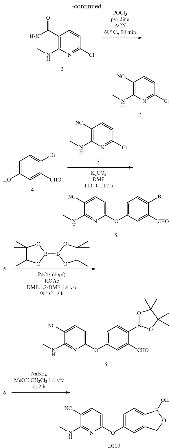
6-Chloro-2-methylamino-nicotinamide (2)
