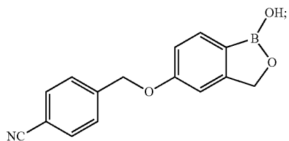
4-(1-Hydroxy-1,3-dihydro-benzo[c][1,2]oxaborol-5-yloxy)-benzoic acid methyl ester
