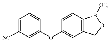
1,3-Dihydro-1-hydroxy-5-(3-cyanophenoxy)-2,1-benzoxaborole
