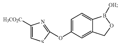
2-(1-Hydroxy-1,3-dihydro-benzo[c][1,2]oxaborol-5-yloxy)-thiazole-4-carboxylic acid methyl ester
