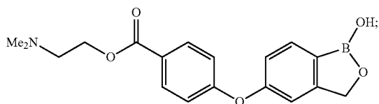
4-(1-Hydroxy-1,3-dihydro-benzo[c][1,2]oxaborol-5-yloxy)-benzoic acid 2-dimethylamino-ethyl ester
