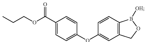
4-(1-Hydroxy-1,3-dihydro-benzo[c][1,2]oxaborol-5-yloxy)-benzoic acid propyl ester
