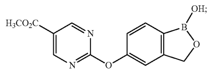
2-(1-Hydroxy-1,3-dihydro-benzo[c][1,2]oxaborol-5-yloxy)-thiazole-4-carboxylic acid methyl ester
