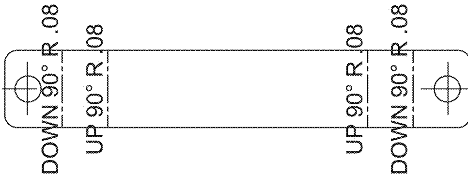
FLAT PATTERN FIG. 9B
