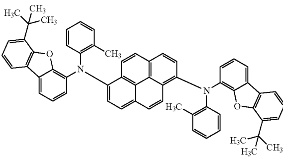
Compound 7
