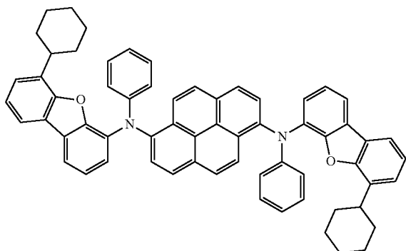
Compound 6
