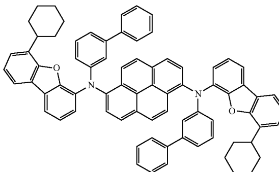
Compound 8
