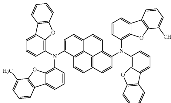
Compound 9
