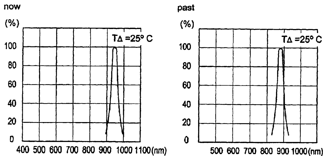
The spectral curve of the LED
