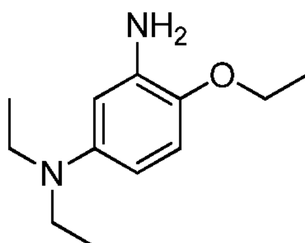
aniline 18
