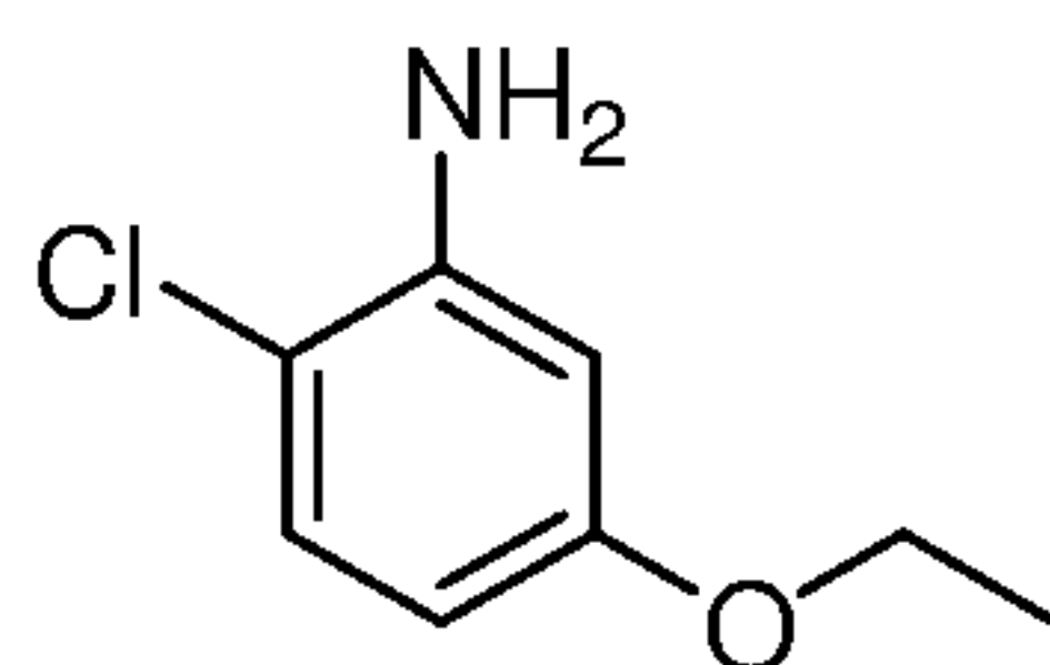
aniline 14
