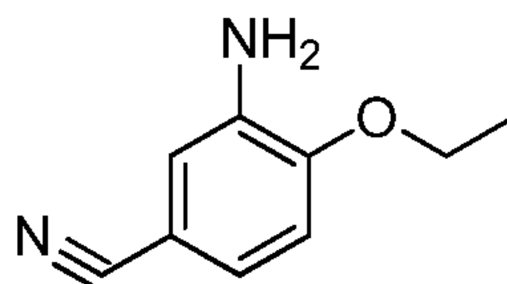
aniline 21
