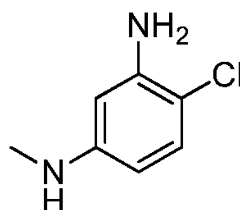
aniline 20
